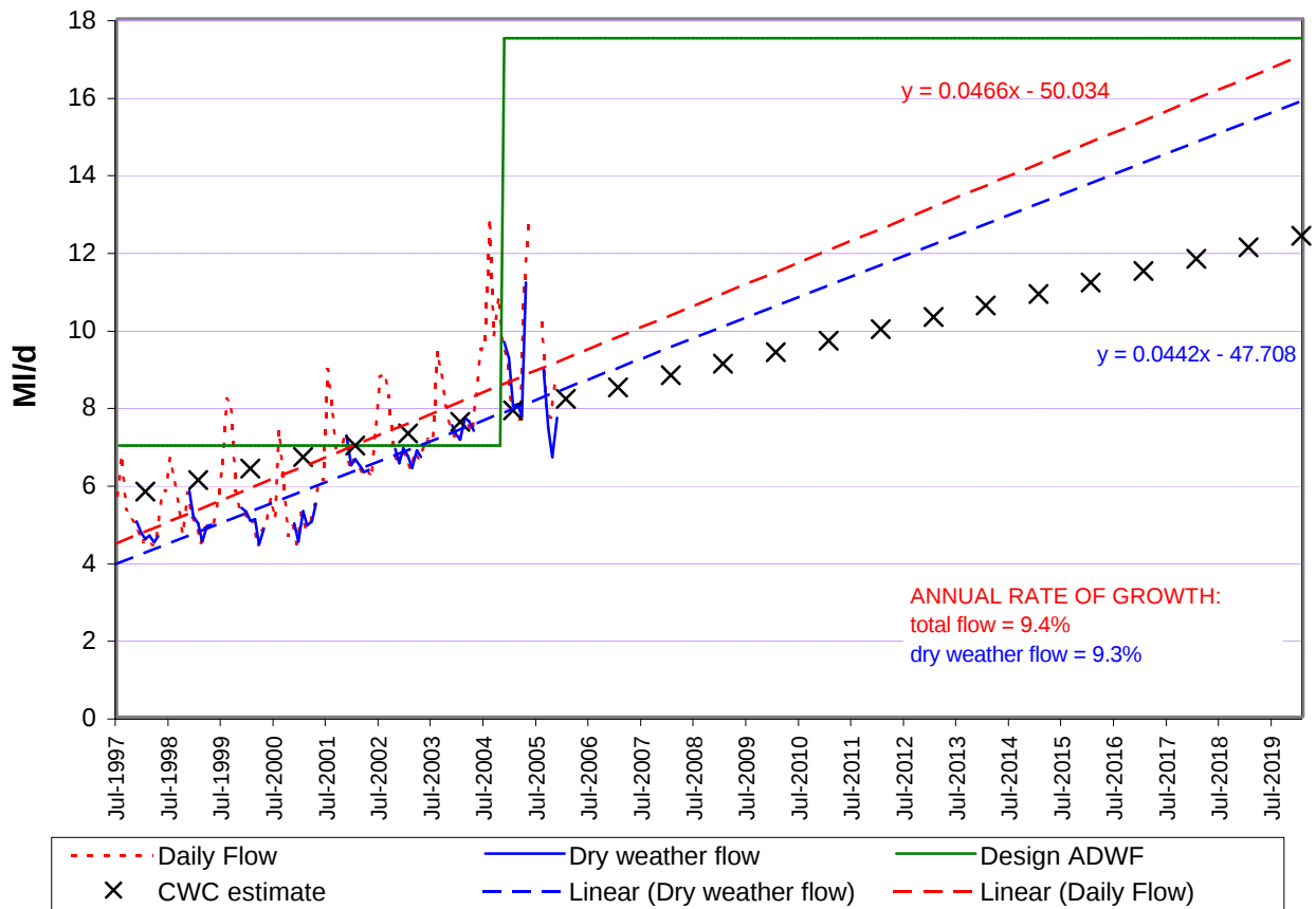
KRAAIFONTEIN WWTW: FLOW
