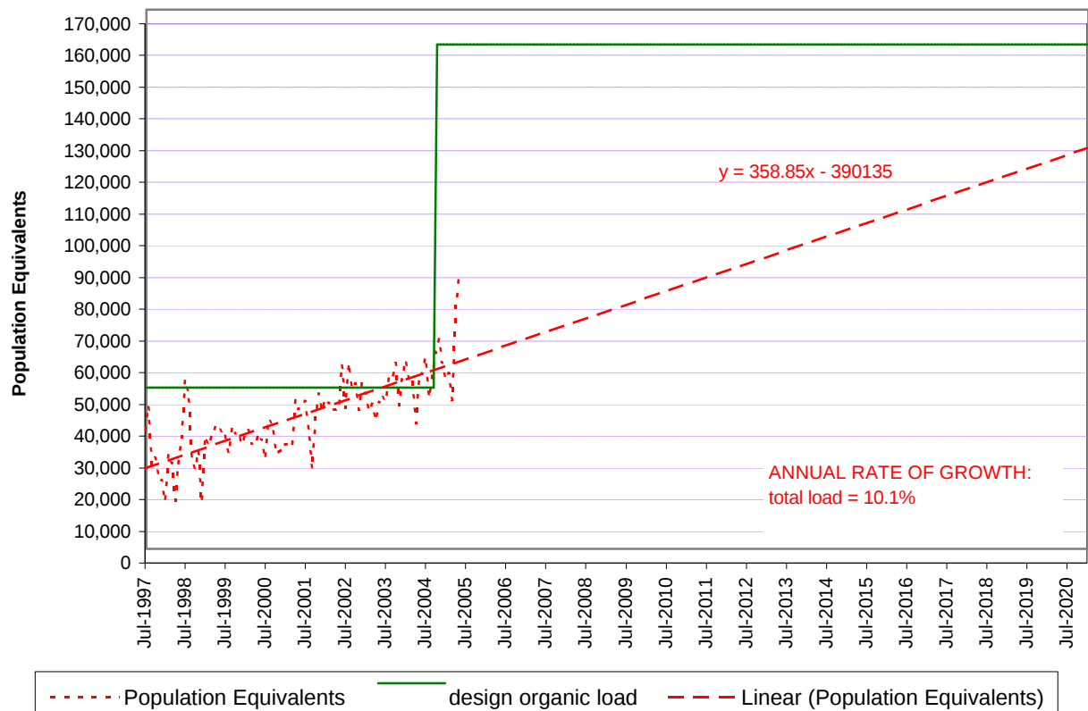
KRAAIFONTEIN WWTW: ORGANIC LOAD
