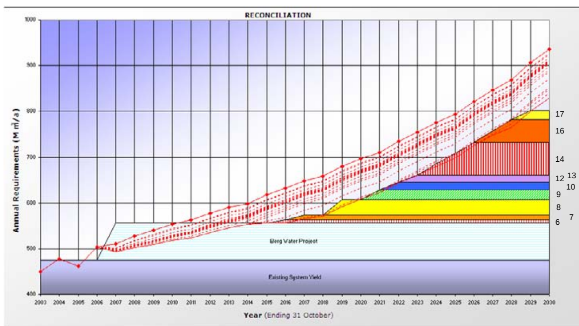
Figure 3.8 Scenario 7: CCT WC/WDM strategy and lowest URV supply-side and WC/WDM interventions
