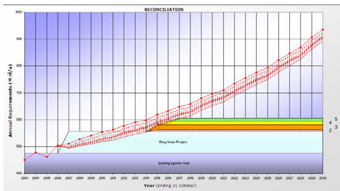
Figure 3.2 Scenario 2: No additional WC/WDM interventions and all supply-side interventions
