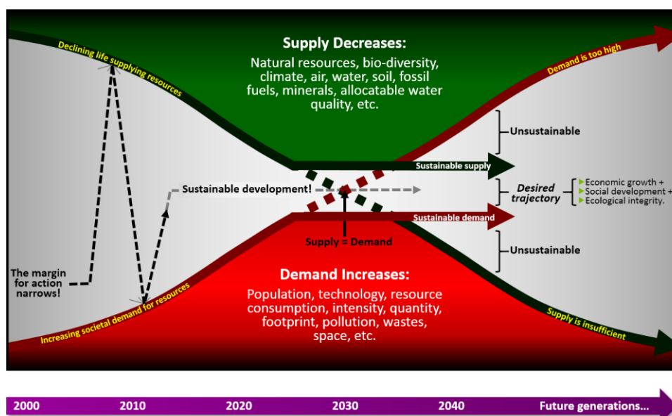
FIGURE 26: Natural Step Funnel demonstrating converging global supply & demand [Adapted from The Natural Step].
