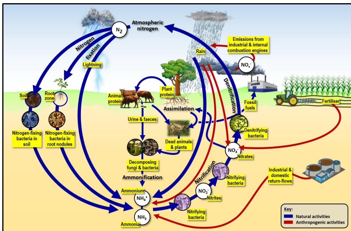
FIGURE 13: The bio-geochemical nitrogen cycle.
