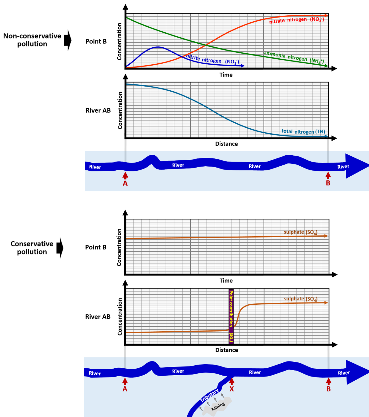
FIGURE 22: A comparison between non-conservative and conservative pollution, depicting nitrogen, in the context of nitrogen cycling, and sulphate on concentration-over-time, and concentration-over-distance graphs.
