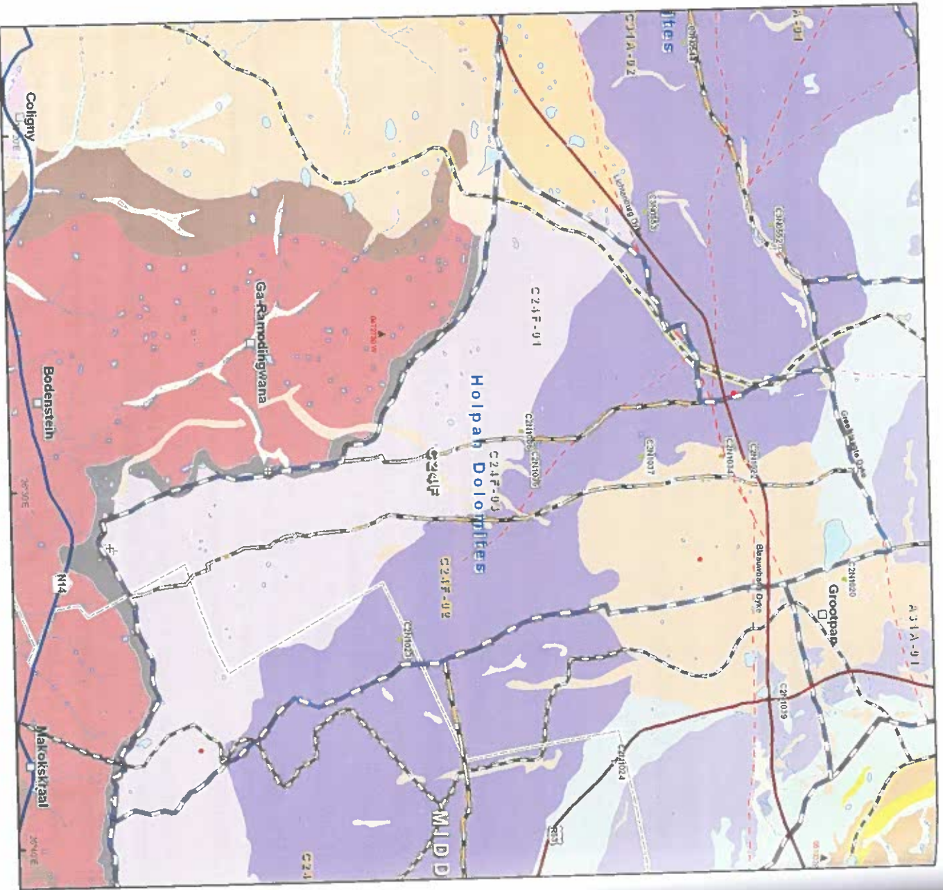
Figure 7.13. Map showing the outline of the Holpan GMA (from Holland, 2009).
