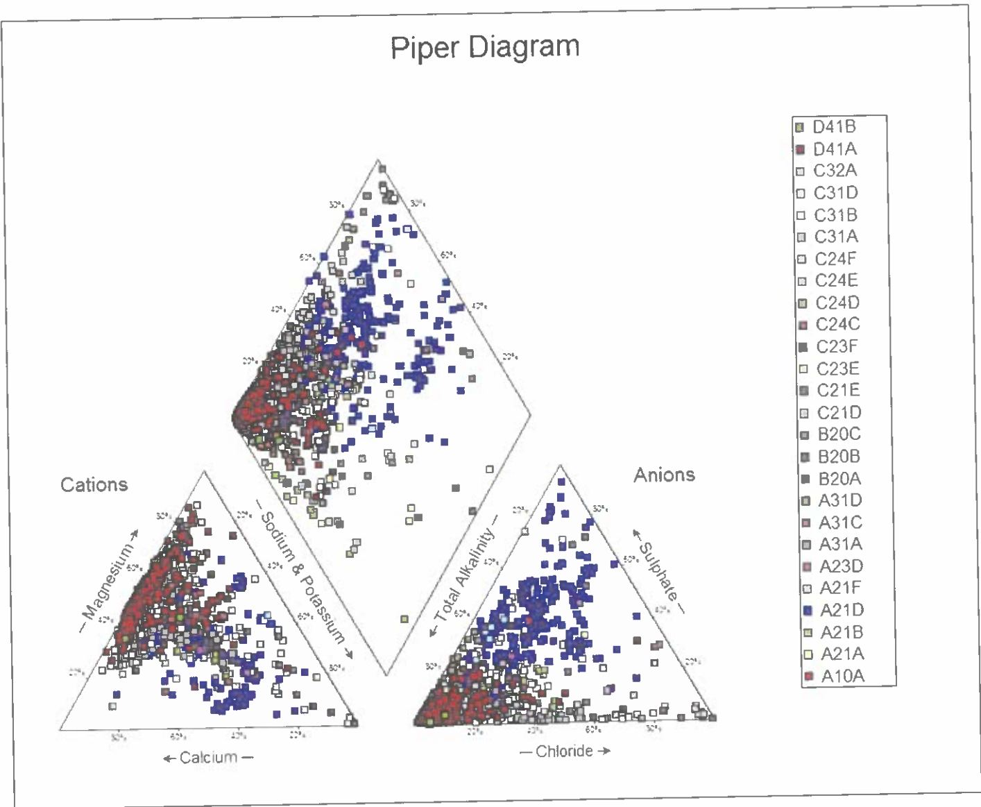
Figure 14.2: Piper diagram of water quality according the Quaternary catchments.
