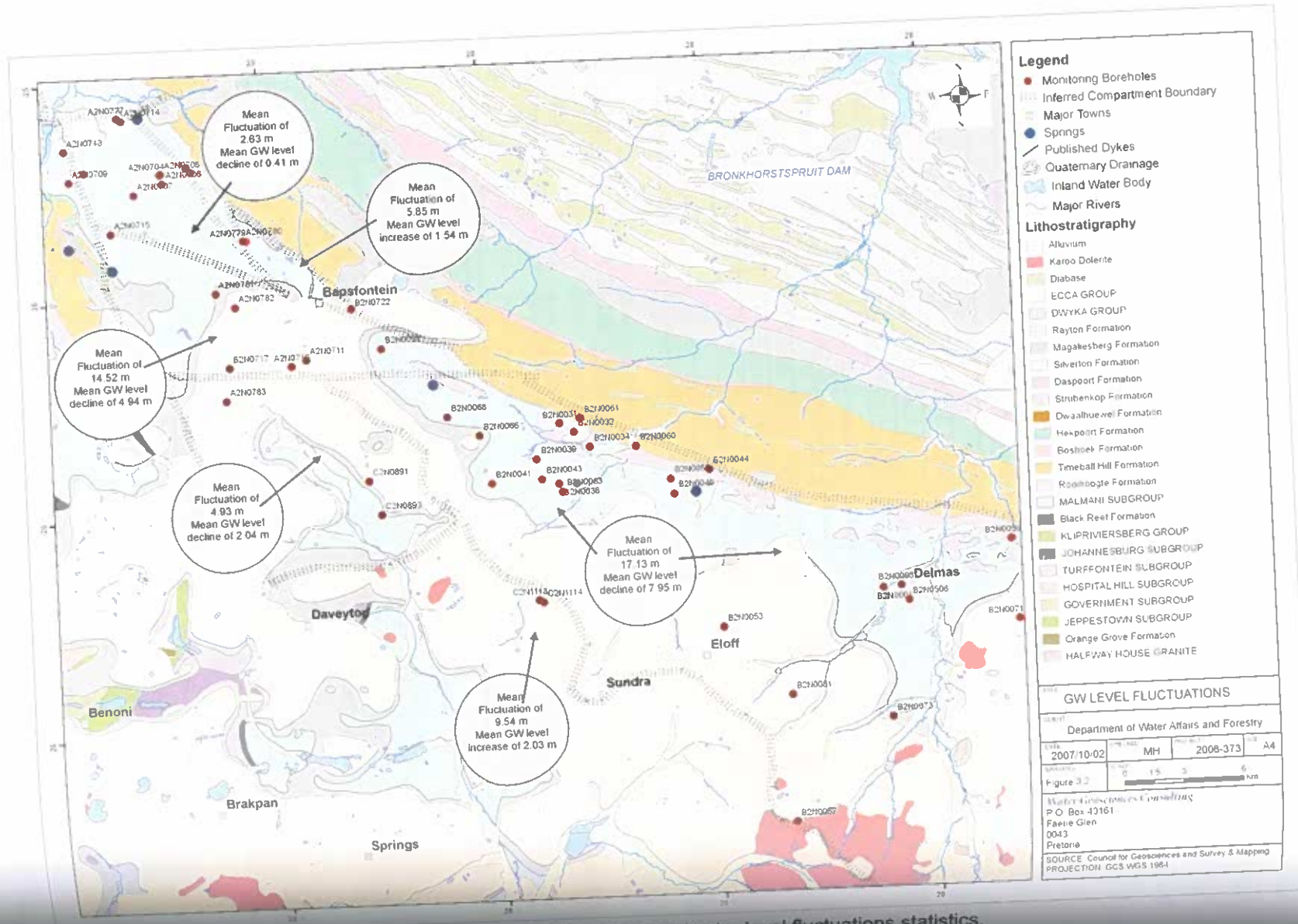
Figure 11.7. Spatial view of groundwater level fluctuations statistics.
