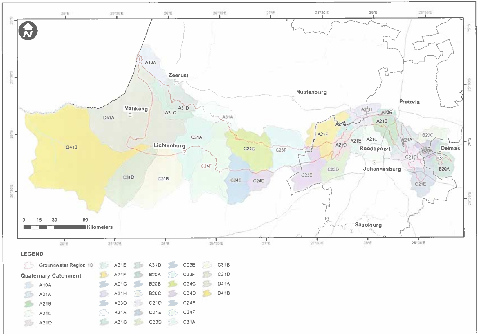
Figure 2.2: Map of Groundwater Region 10 displaying the Quaternary catchment areas in and around the region.
