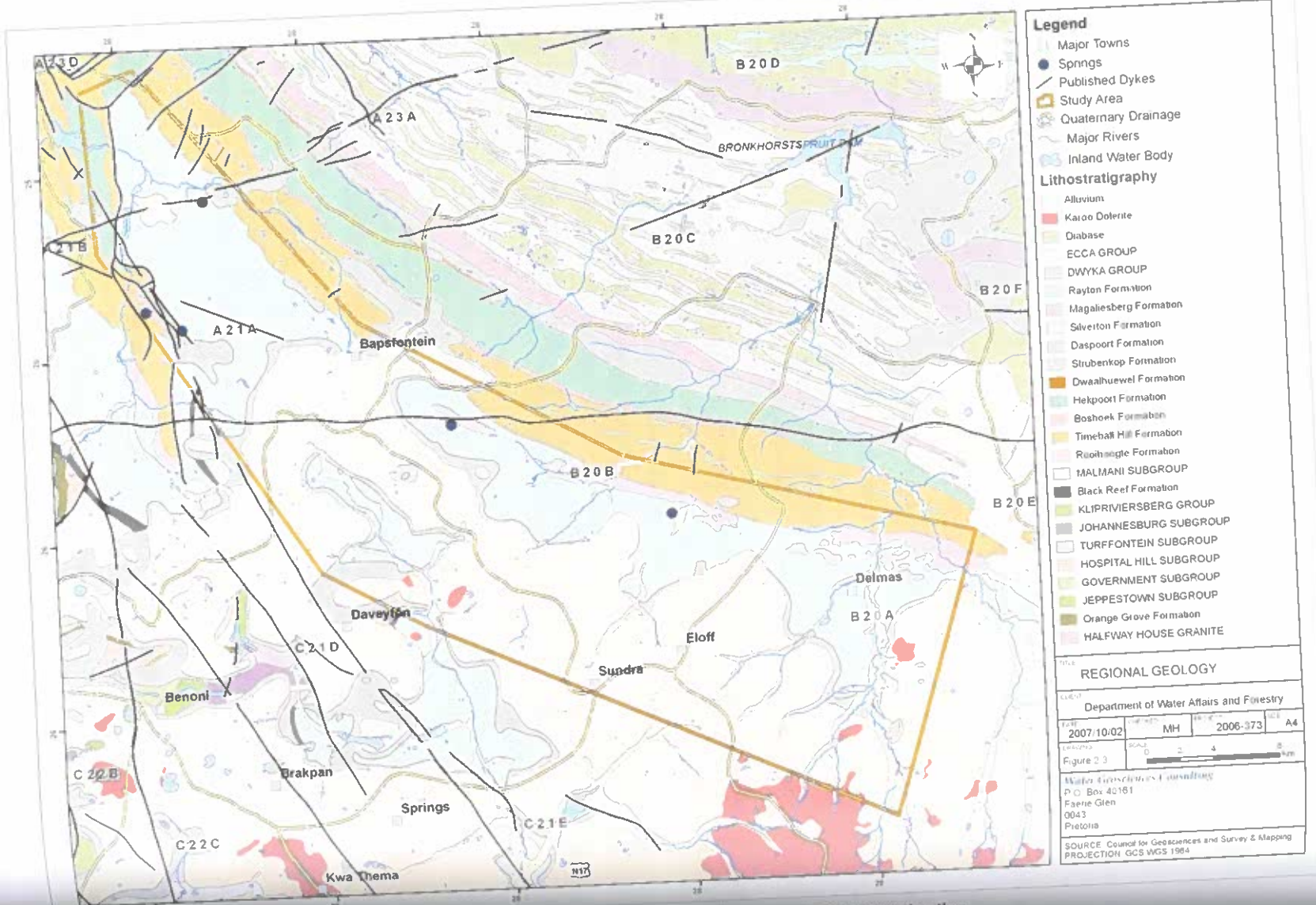
Figure 11.4. Regional geology of the area under investigation.
