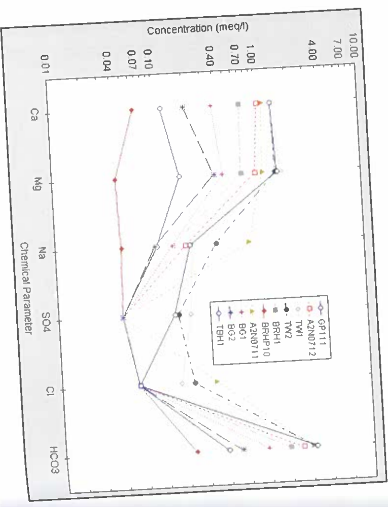
Figure 11.14. Characterisation of groundwater samples (2005) for the Bapsfontein town area.
