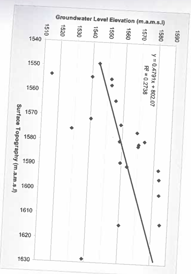
Figure 11.10. Correlation between surface topography and groundwater levels in the Delmas area.
