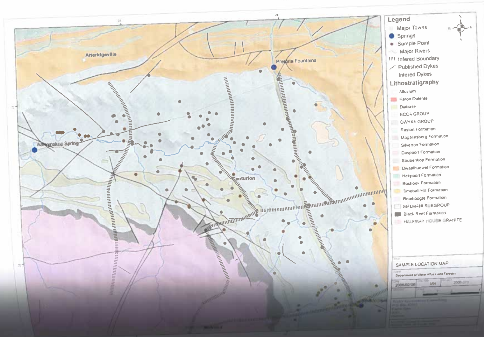
Figure 10.5: Groundwater quality sample locations
