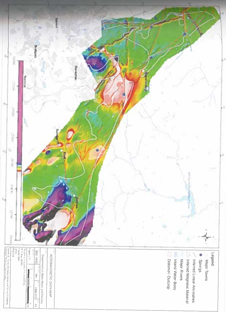
Figure 11.5. Aeromagnetic data interpretation (Sourced from: The Council for Geosciences).
