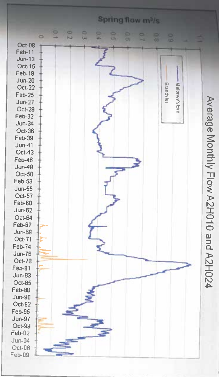
Figure 8.4. Flow hydrographs of DWAf gauging stations A2H010 and A2H024.
