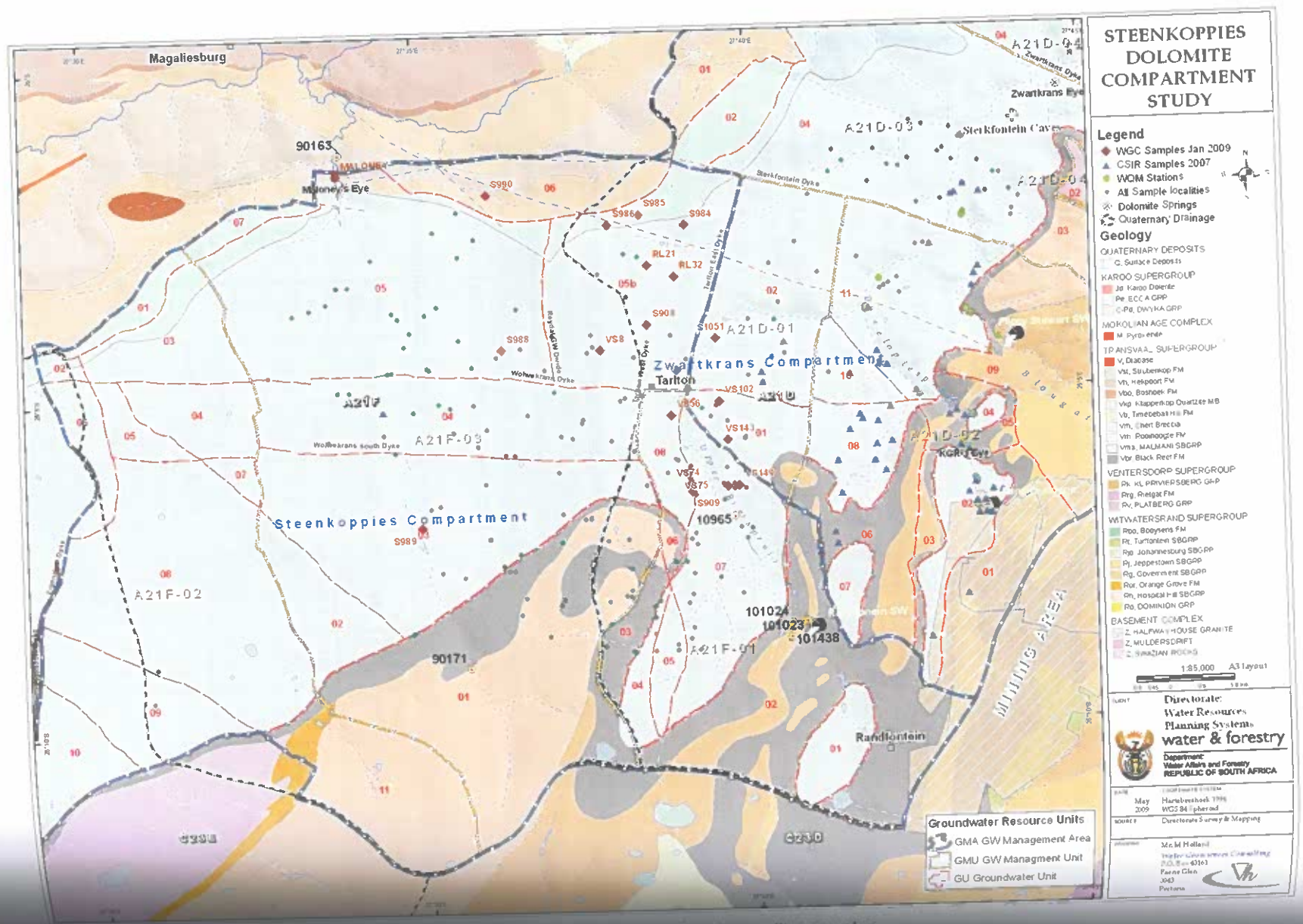
Figure 8.21. Distribution of water quality samples.
