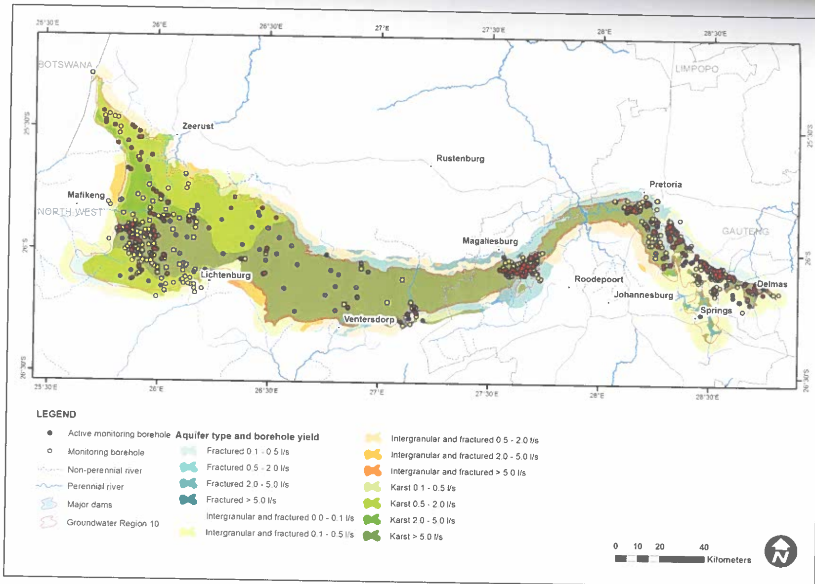
Figure 7.20. Aquifer type and borehole yield across Groundwater Region 10.
