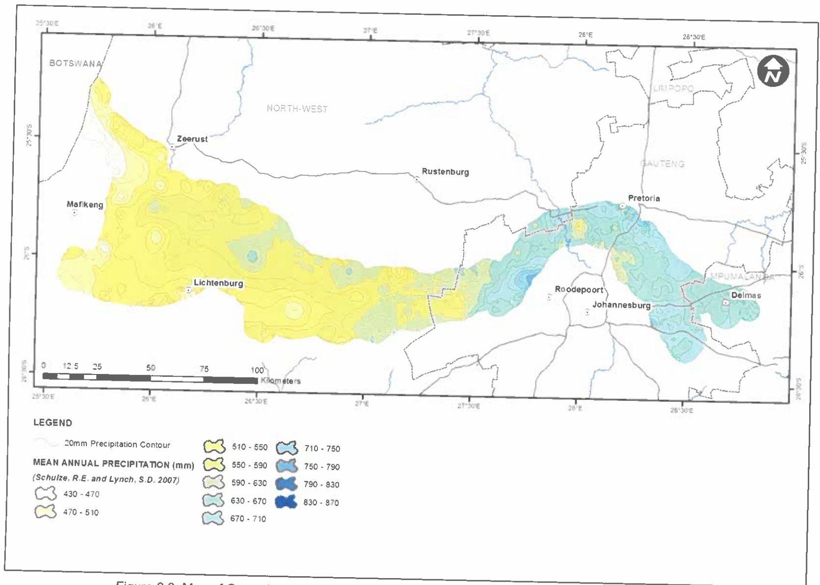
Figure 2.3: Map of Groundwater Region 10 displaying Mean Annual Precipitation across the Region
