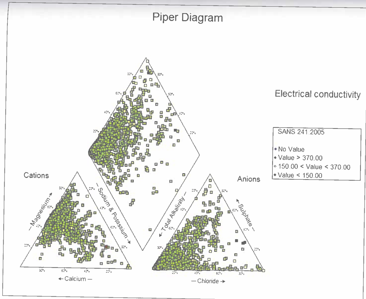
Figure 14.1: Piper diagram based on Electrical Conductivity groupings
