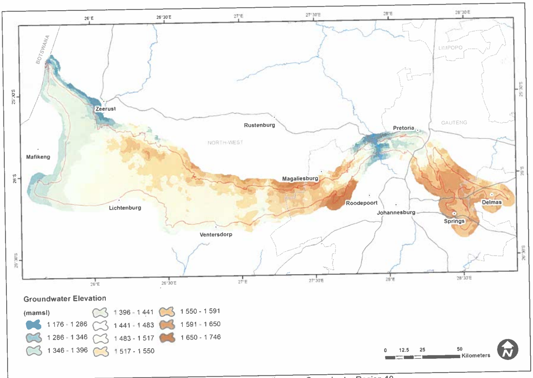
Figure 7.17. Groundwater level elevation (mamsl) across Groundwater Region 10.
