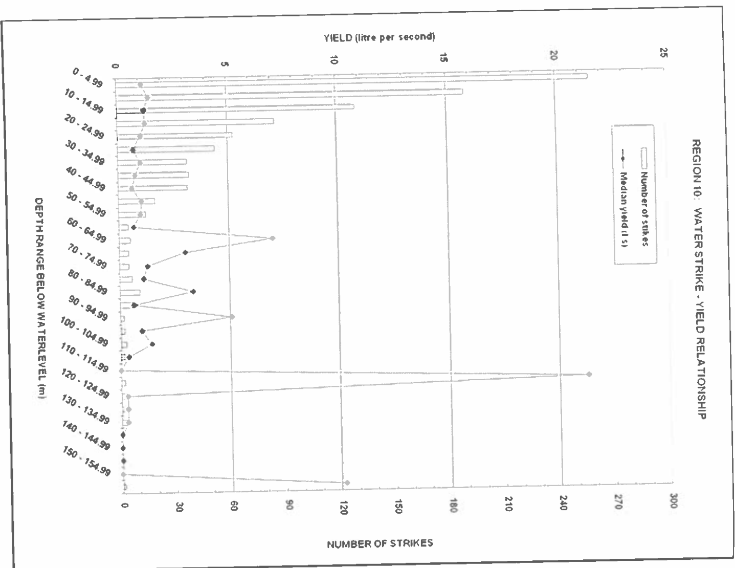
Figure 12.5: Borehole yield statistics for Groundwater Region 10.
