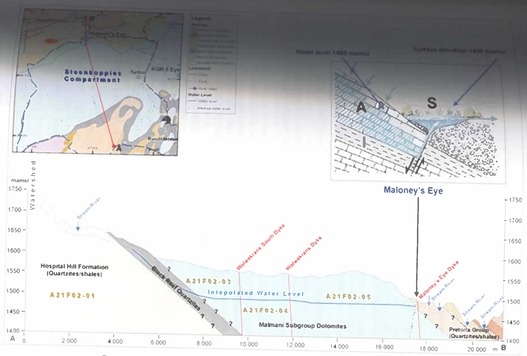
Figure 8.30. Conceptual model of the Maloney's Eye based on a south-north cross section.
