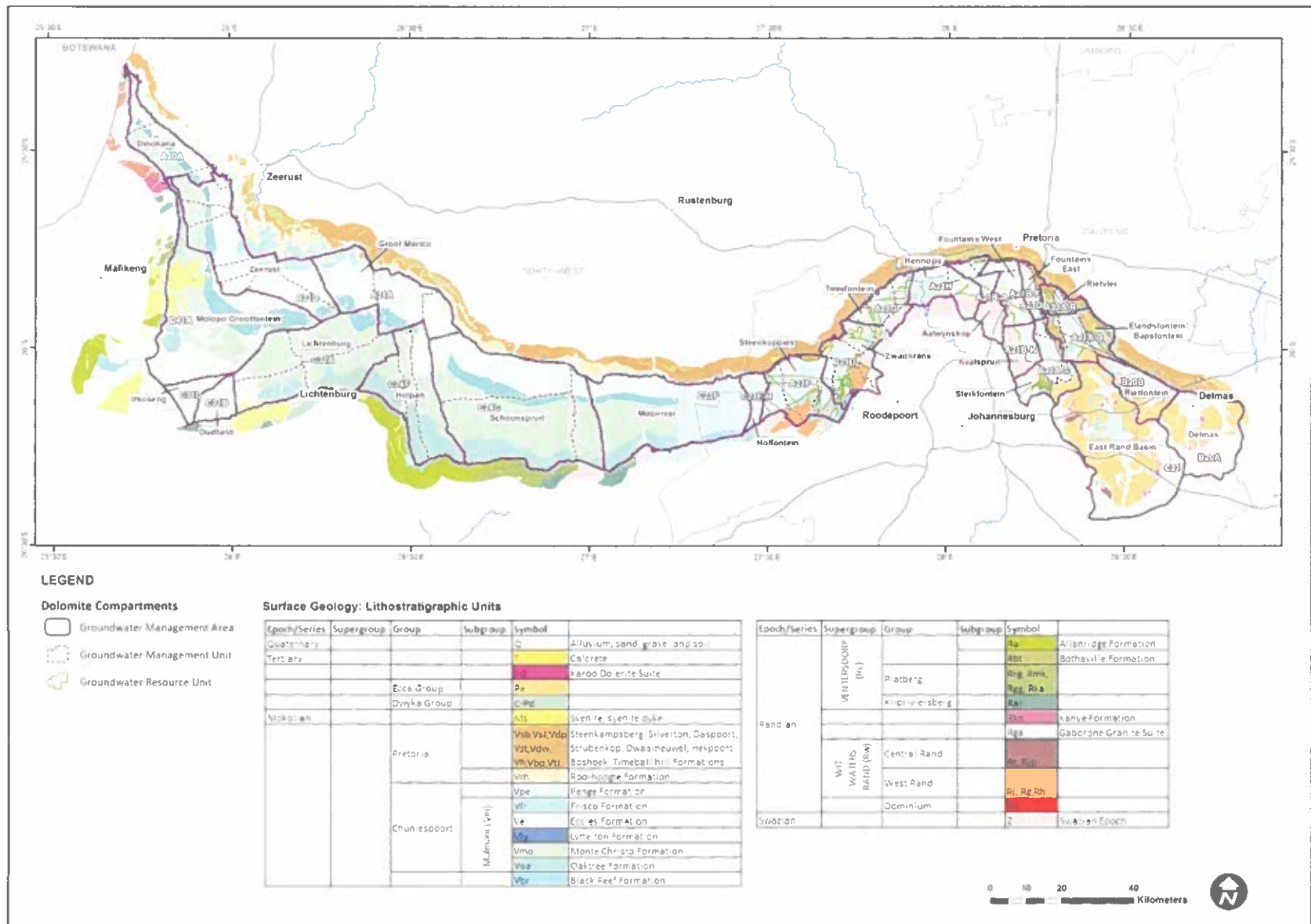
Figure 6.1: Map of Region 10 showing the boundaries to the different GMAs or compartments.
