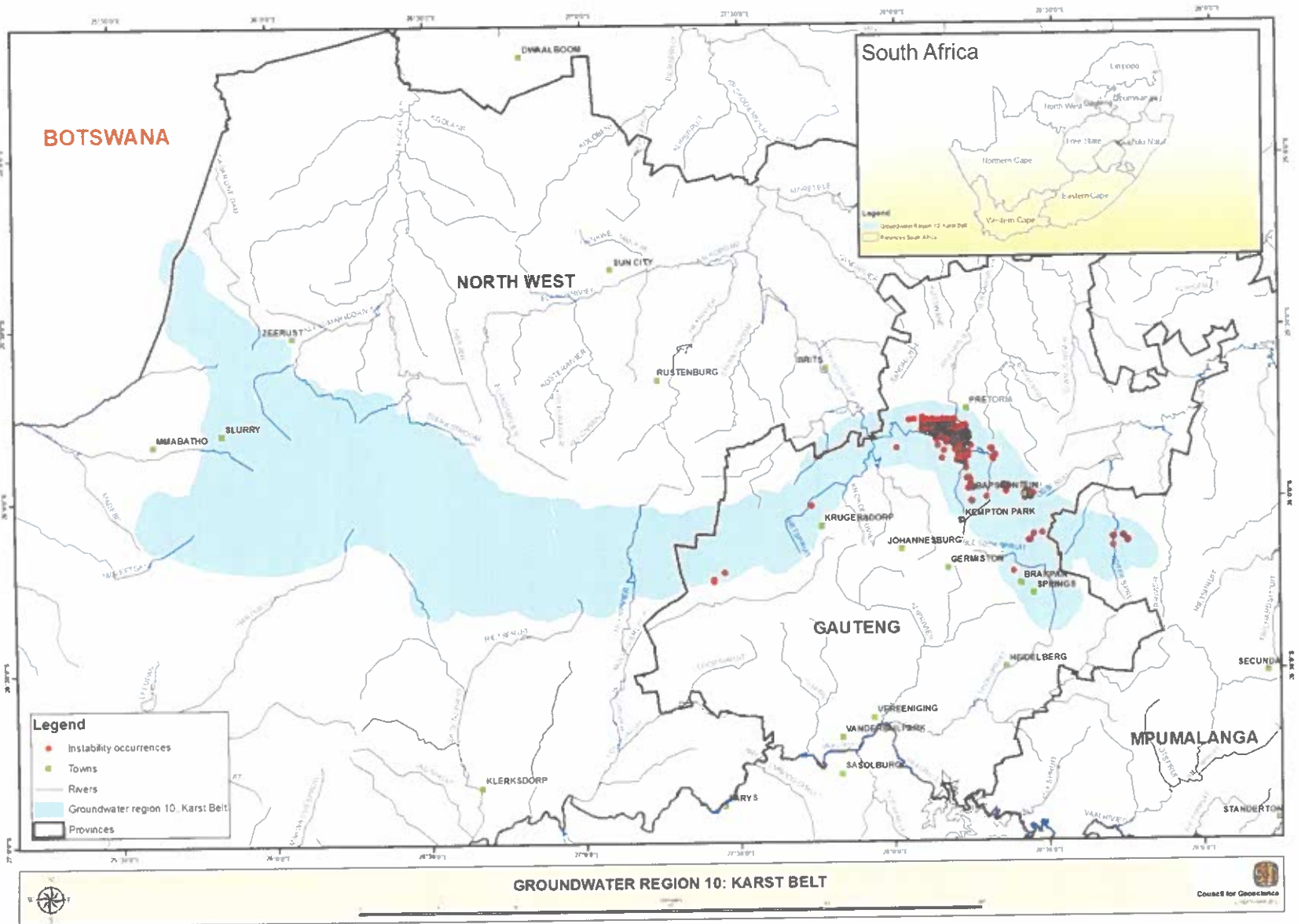
Figure 4.4: Sinkhole and subsidence occurrences across Groundwater Region 10 (Data provided with courtesy of the Council for Geoscience, Pretoria).
