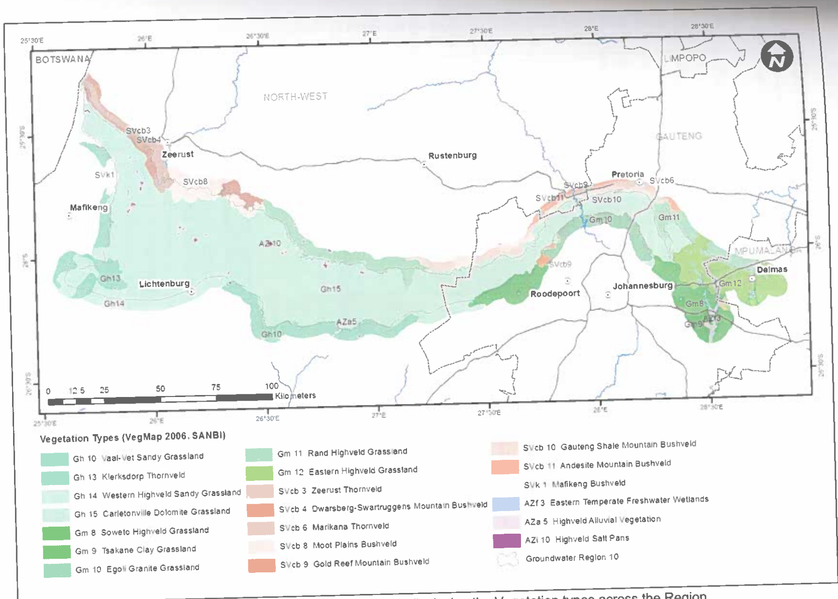
Figure 2.4: Map of Groundwater Region 10 displaying the Vegetation types across the Region.
