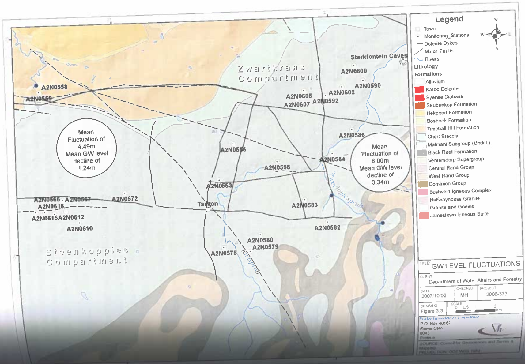
Figure 9.8 Spatial view of groundwater level monitoring stations and compartment fluctuations statistics
