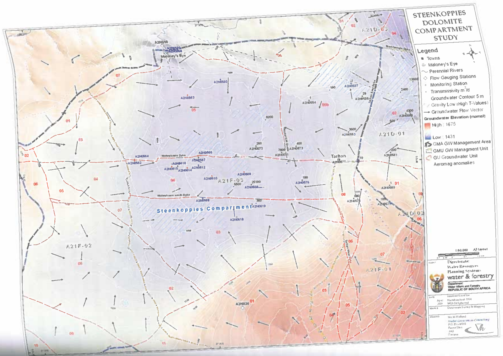
Figure 8.10 Regional groundwater flow.
