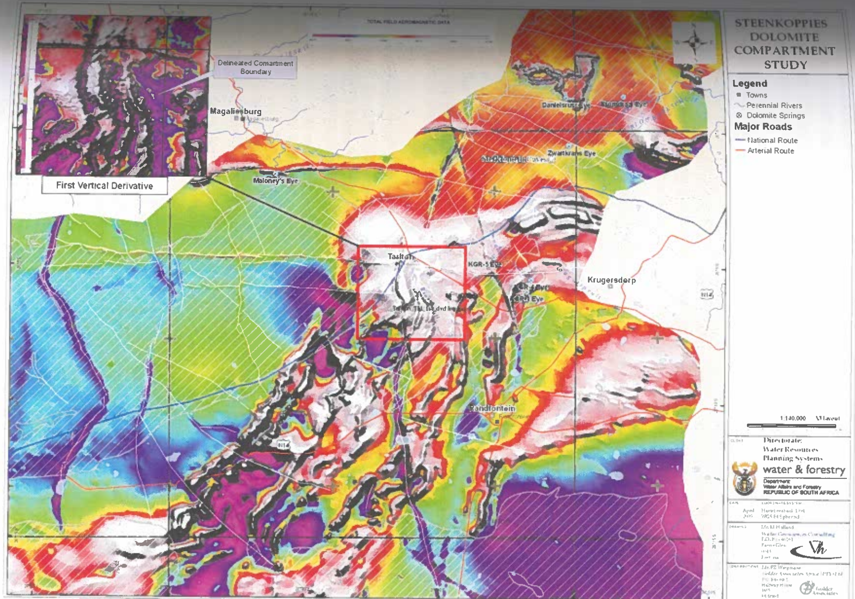
Figure 8.7. Aeromagnetic data interpretation (sourced from: The Council for Geosciences by Holland, 2009).
