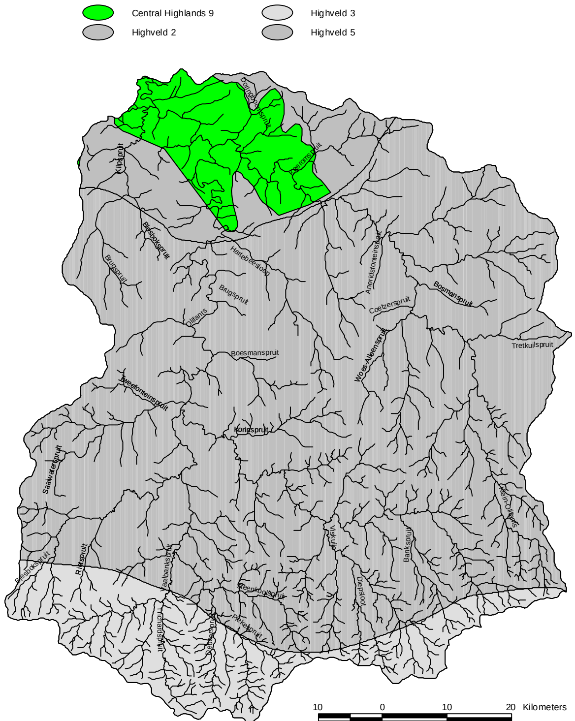
Figure 12. 1:250 000 rivers coverage for DWAF secondary catchment B1 showing ecoregion level 2s.
