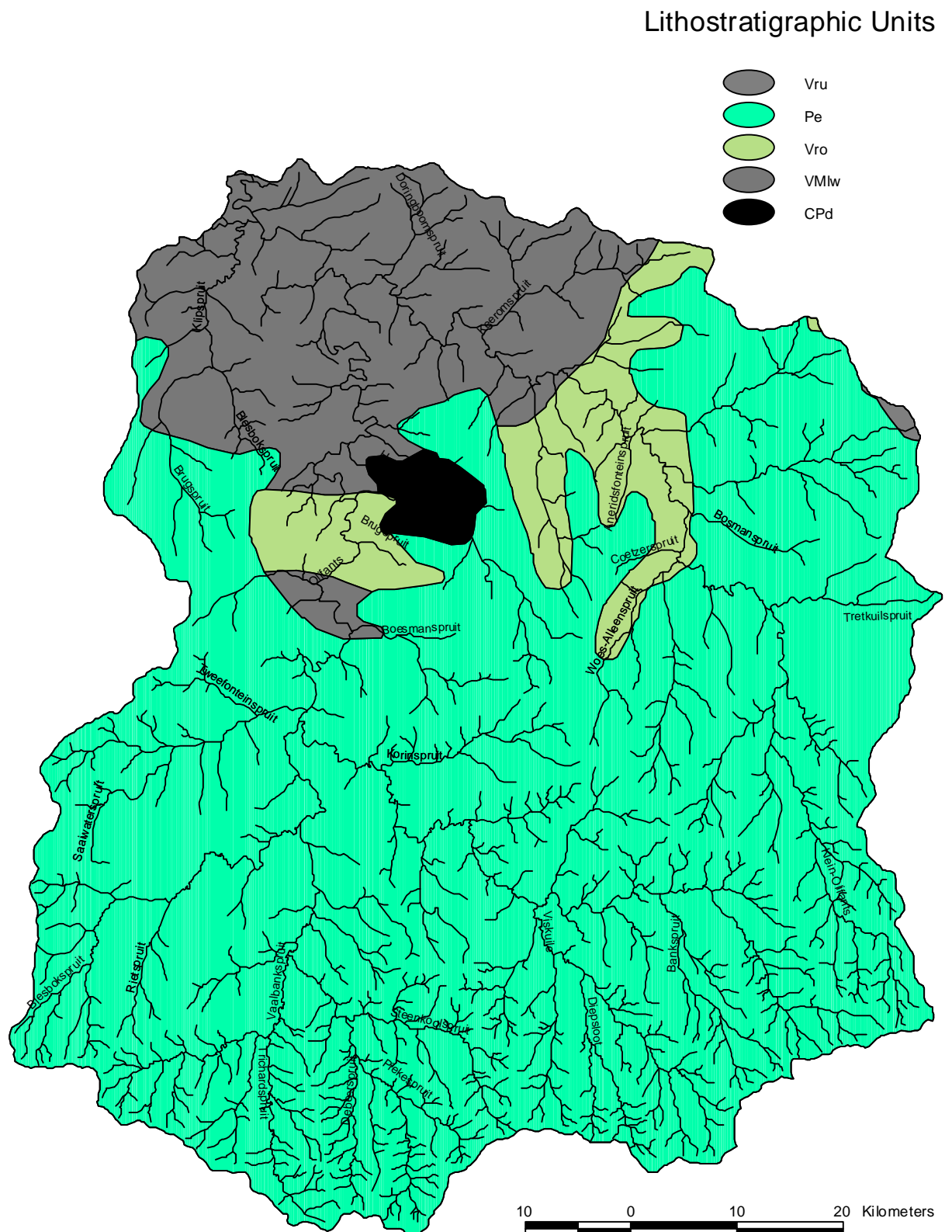
Figure 15. 1:250 000 rivers coverage for DWAF secondary catchment B1 showing lithostratigraphic units (modified from Vegter 1995). Details of the lithostratigraphic units are given in Appendix 2.
