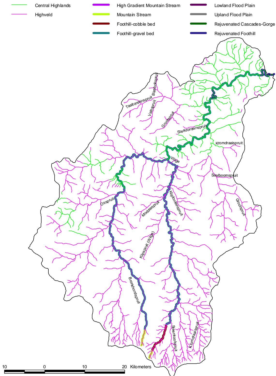
Figure 16. 1:250 000 rivers coverage for DWAF secondary catchment B2 coded by ecoregion level 1s and geomorphological zones.
