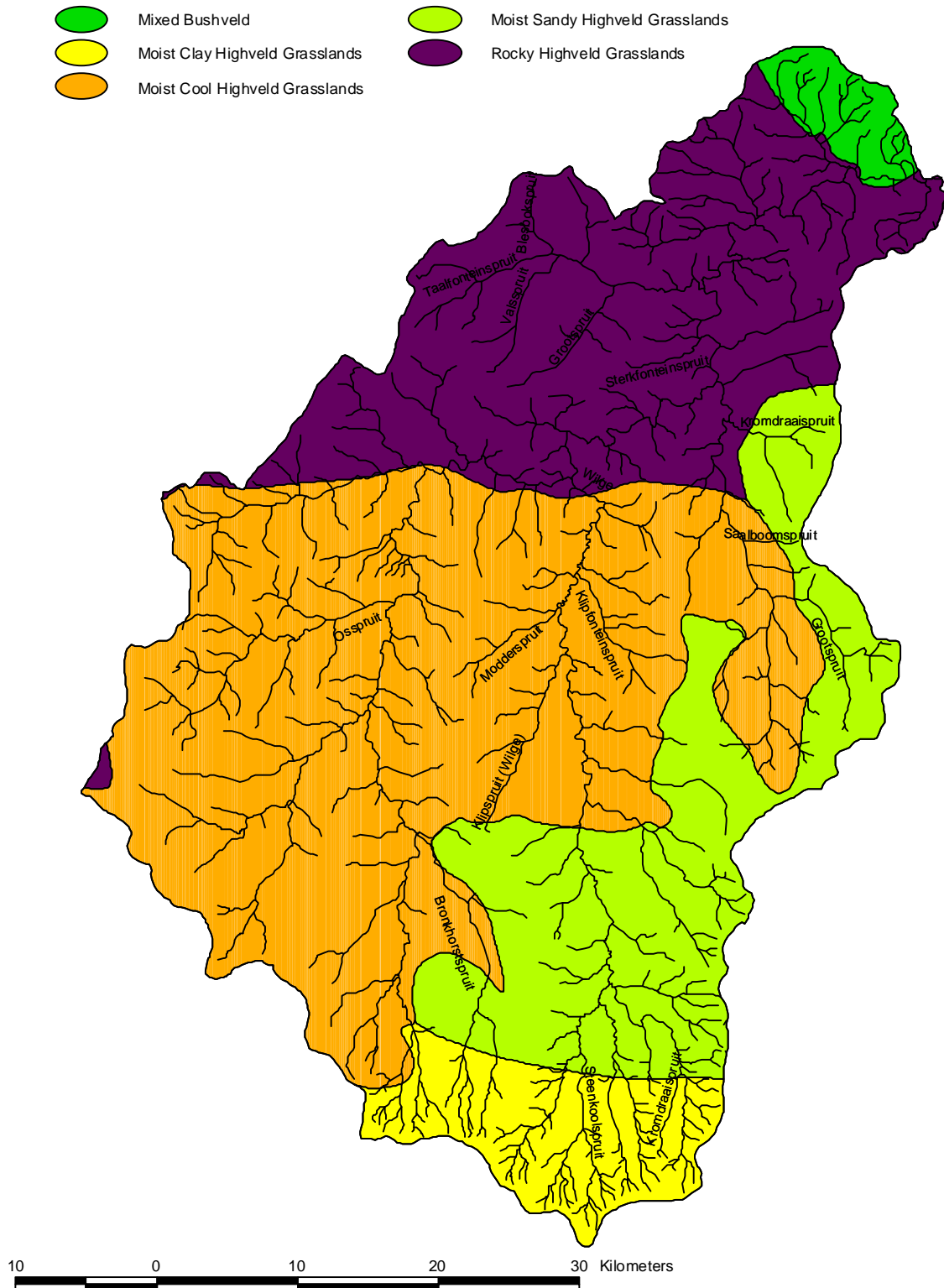
Figure 19. 1:250 000 rivers coverage for DWAF secondary catchment B2 showing potential natural vegetation (modified from Low and Rebelo 1996). Details of the vegetation are given in Appendix 1.
