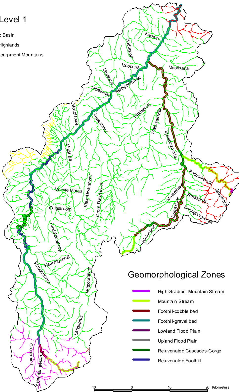
Figure 26. 1:250 000 rivers coverage for DWAF secondary catchment B4 coded by ecoregion level 1s and geomorphological zones.
