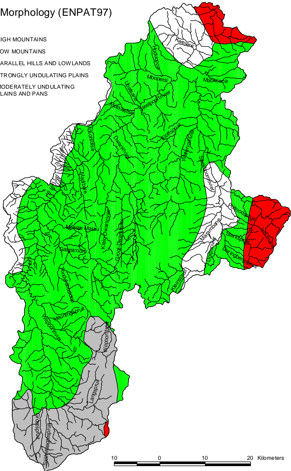
Figure 28. 1:250 000 rivers coverage for DWAF secondary catchment B4 showing terrain morphology (modified from Van Riet et al. 1997).
