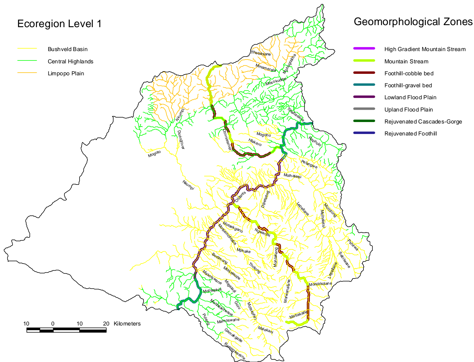
Figure 31. 1:250 000 rivers coverage for DWAf secondary catchment B5 coded by ecoregion level 1s and geomorphological zones.
