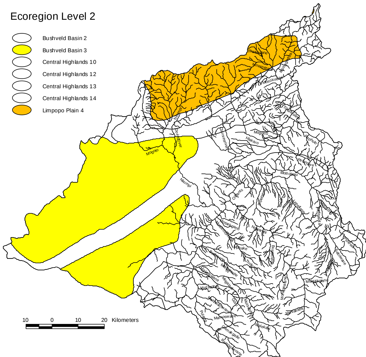
Figure 32. 1:250 000 rivers coverage for DWA secondary catchment B5 showing ecoregion level 2s.
