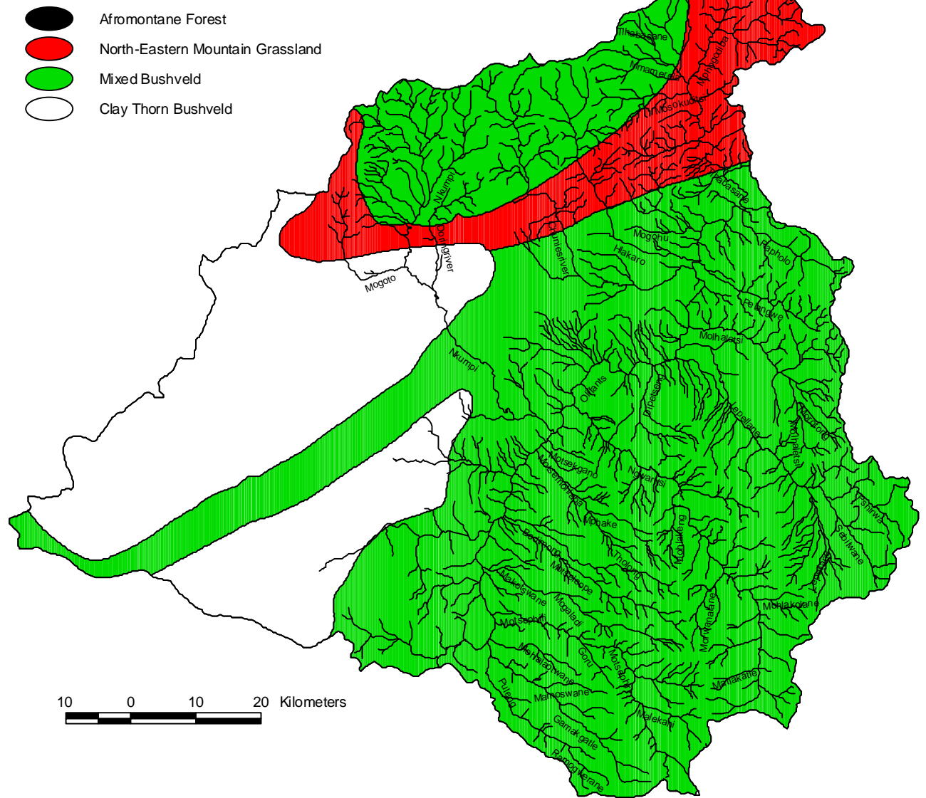
Figure 34. 1:250 000 rivers coverage for DWAF secondary catchment B5 showing potential natural vegetation (Low and Rebelo 1996). Details of the vegetation are given in Appendix 1.
