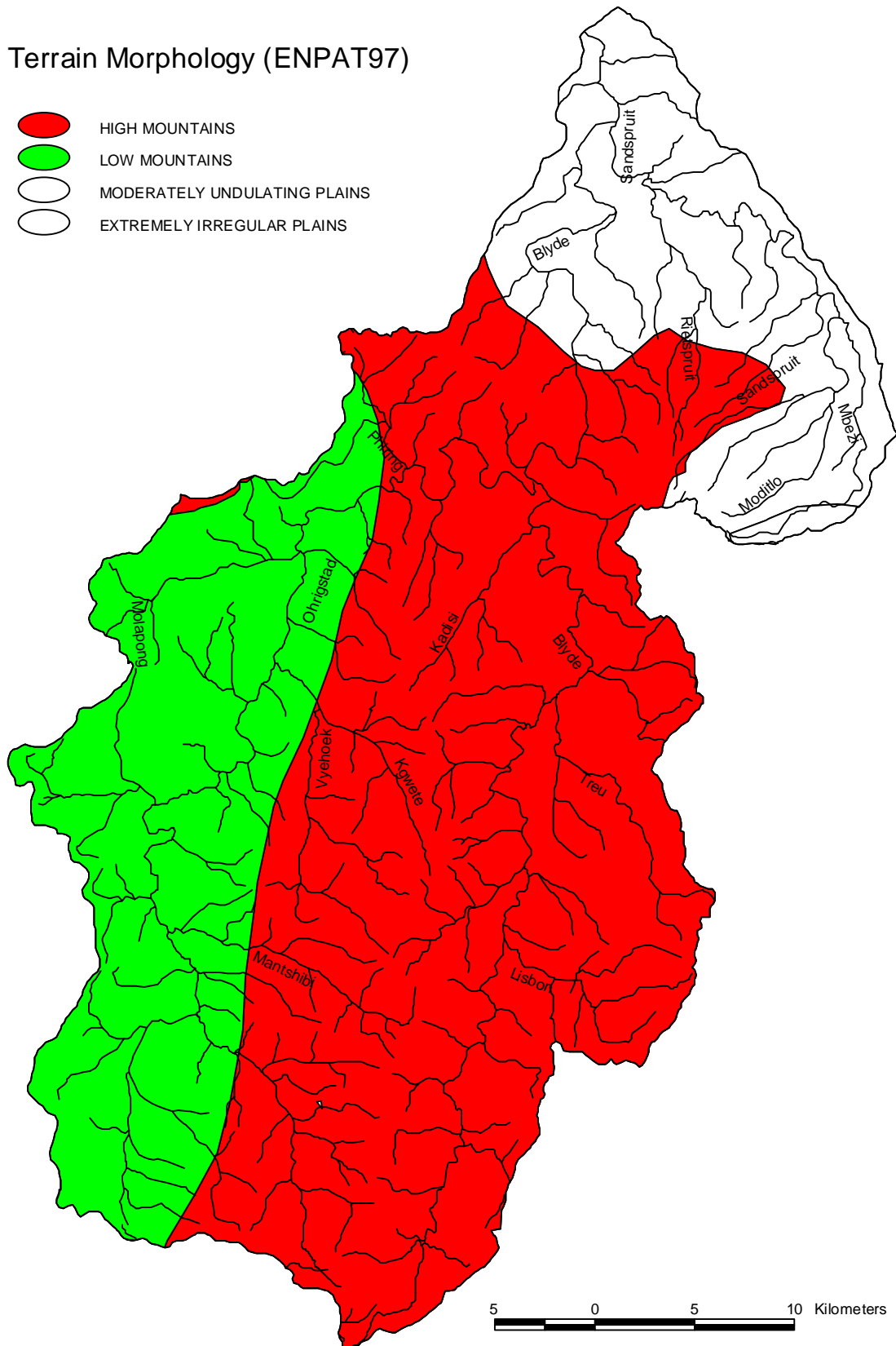
Figure 38. 1:250 000 rivers coverage for DWA secondary catchment B6 showing terrain morphology (modified from Van Riet et al. 1997).
