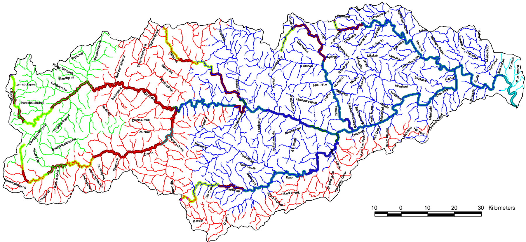
Figure 61. 1:250 000 rivers coverage for DWAF secondary catchment X2 coded by ecoregion level 1s and geomorphological zones.
