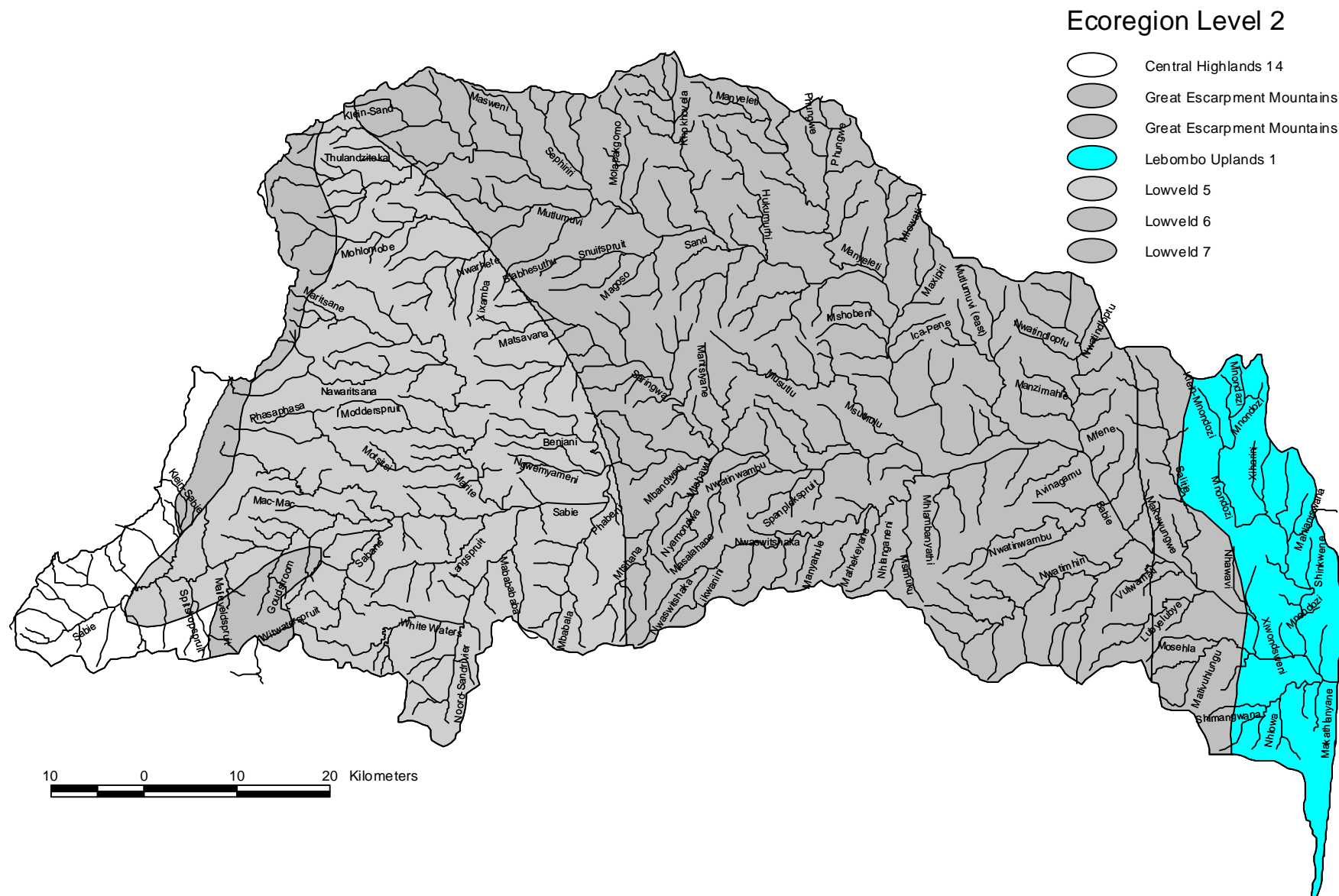
Figure 67. 1:250 000 rivers coverage for DWAf secondary catchment X3 showing ecoregion level 2s.
