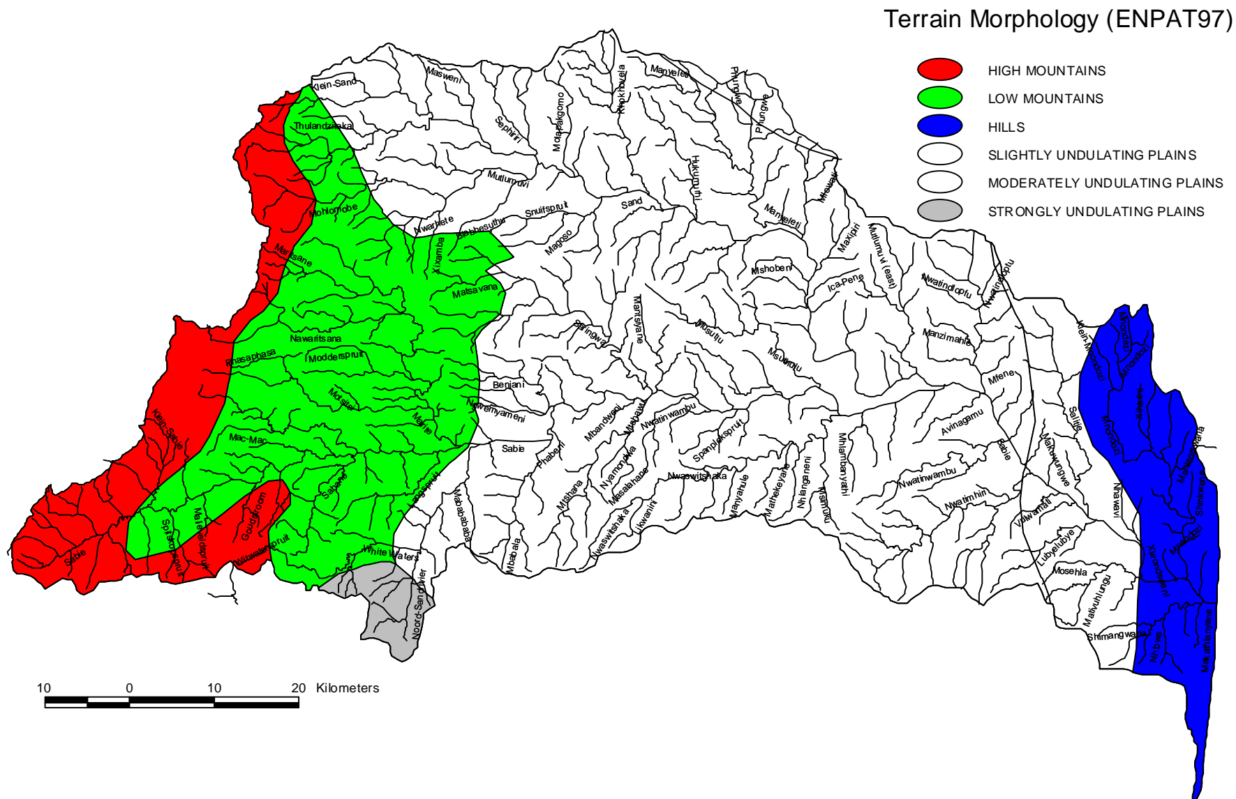
Figure 68. 1:250 000 rivers coverage for DWAF secondary catchment X3 showing terrain morphology (modified from Van Riet et al. 1997).
