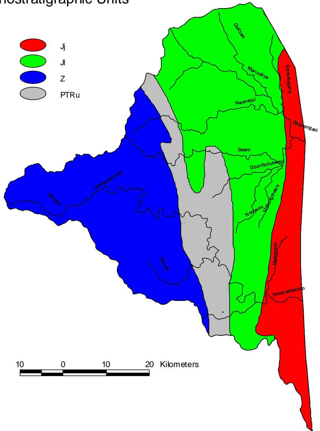
Figure 75. 1:500 000 rivers coverage for DWAF secondary catchment X4 showing lithostratigraphic units (modified from Vegter 1995). Details of the lithostratigraphic units are given in Appendix 2.
