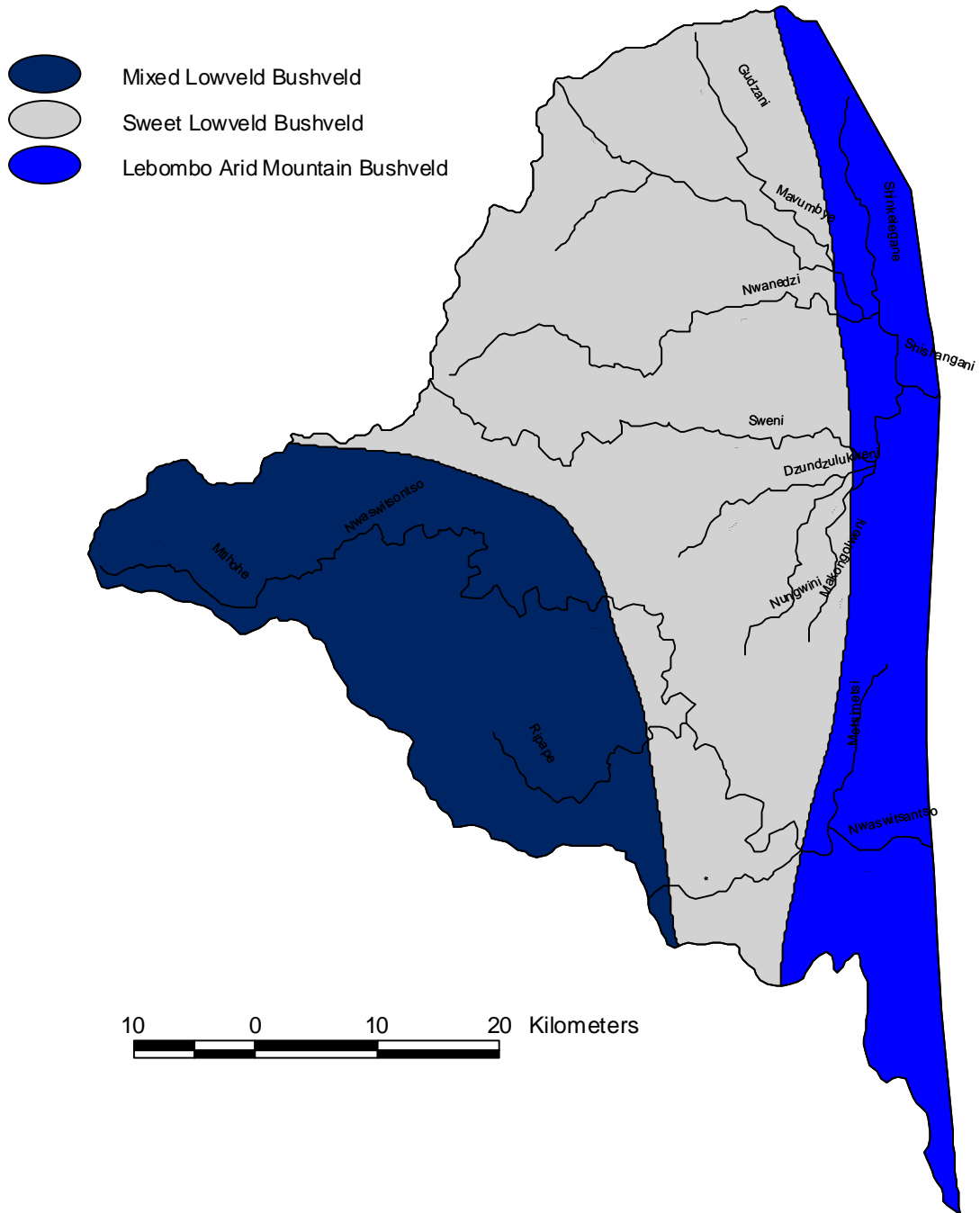
Figure 74. 1:500 000 rivers coverage for DWAF secondary catchment X4 showing potential natural vegetation (modified from Low and Rebelo 1996). Details of the vegetation are given in Appendix 1.
