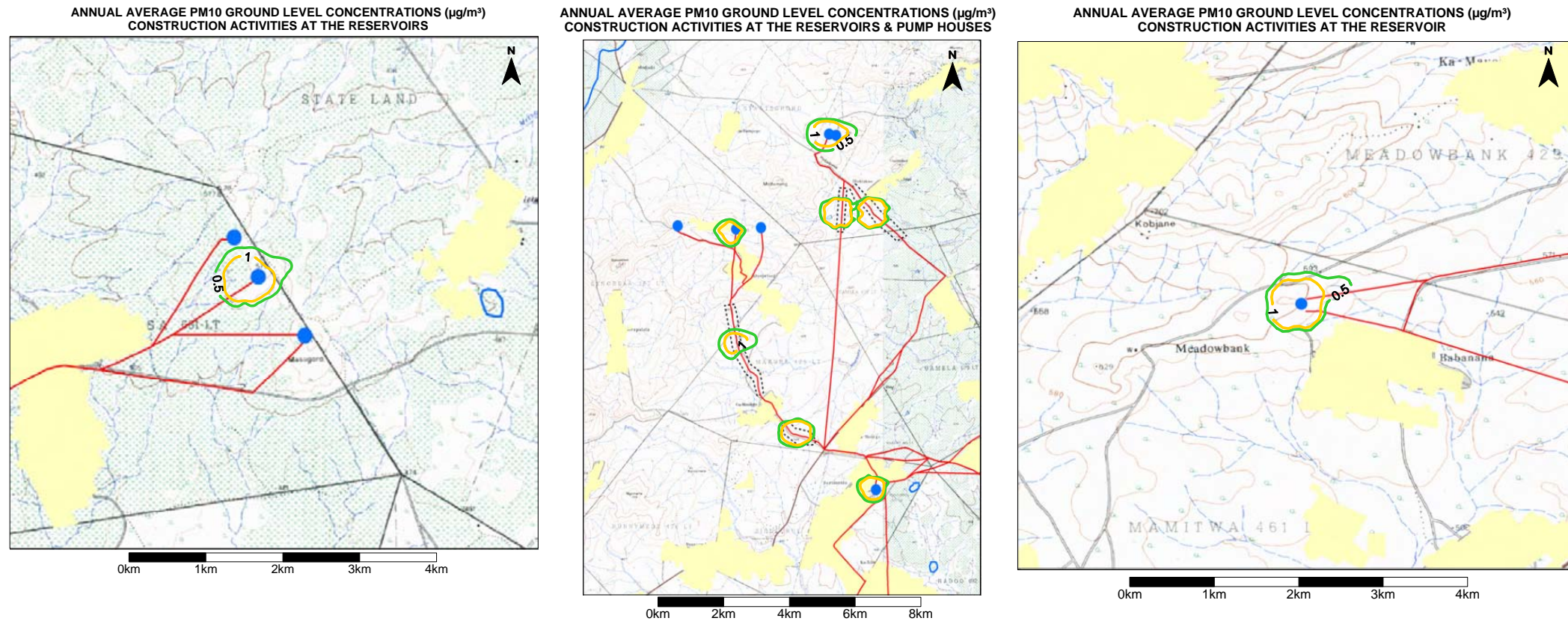
Figure 8.8: Construction of reservoirs and pump houses – annual average PM10 ground level concentrations (µg/m³) (unmitigated).
