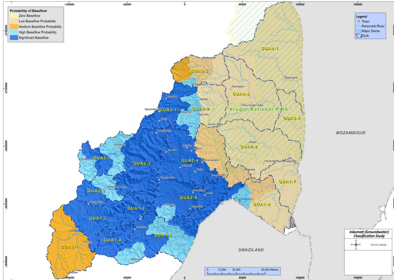
Figure 3.4 Groundwater contribution to baseflow probability.
