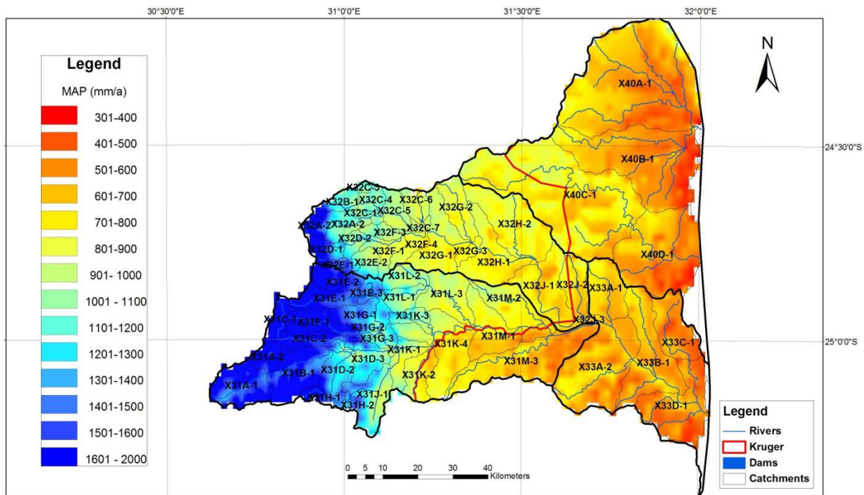
Figure 2.3 Rainfall in the Sabie catchment (DWA, 2009c)
