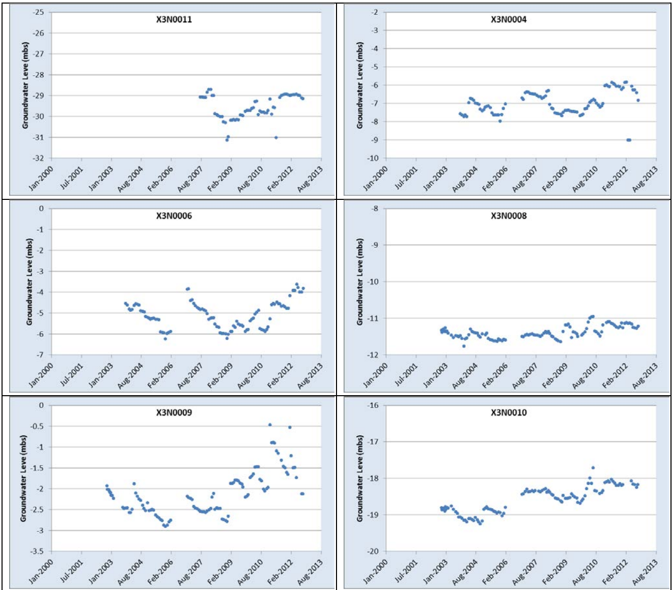
Selected water level monitoring trends for the Sabie/Sand Sub-Catchment
