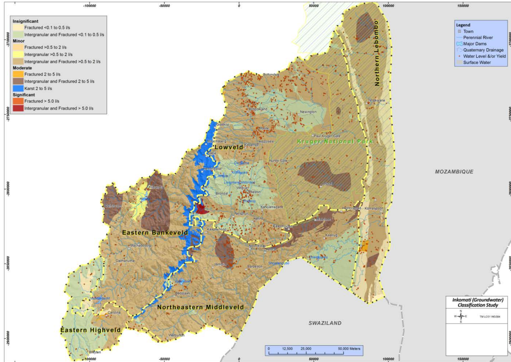
Figure 3.2 Groundwater regions and aquifer yields for the Inkomati WMA.
