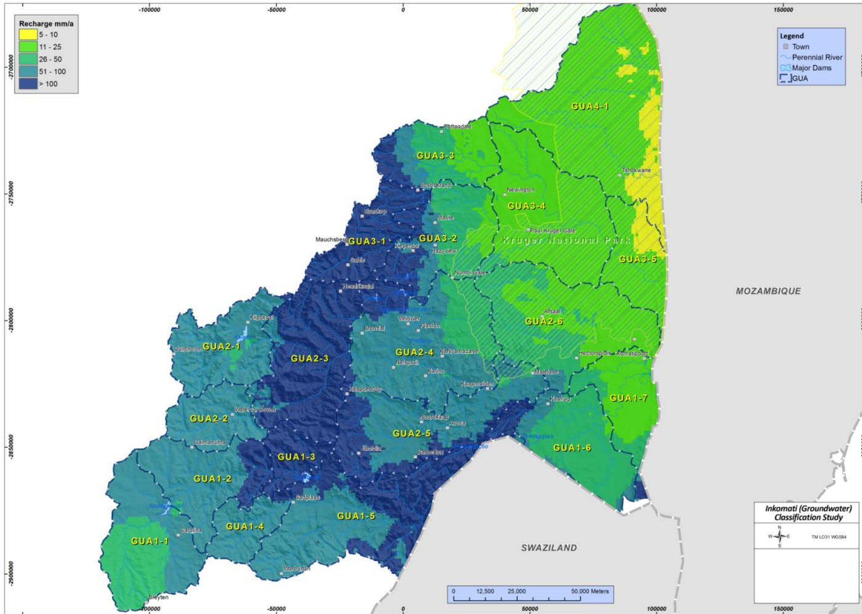
Figure 3.5 Recharge distribution map based on values obtained from the GRA II dataset.
