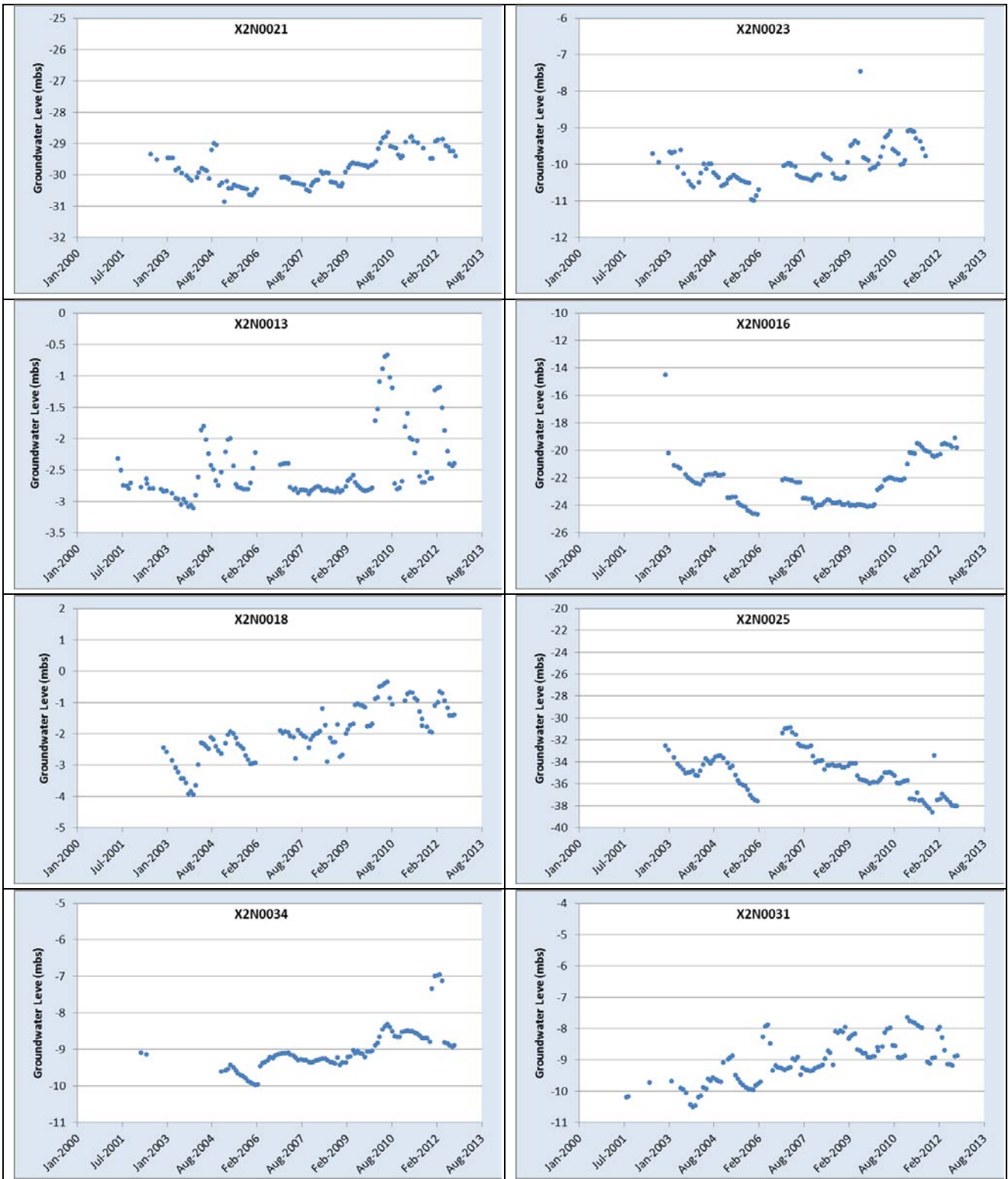
Selected water level monitoring trends for the Crocodile Sub-Catchment.
