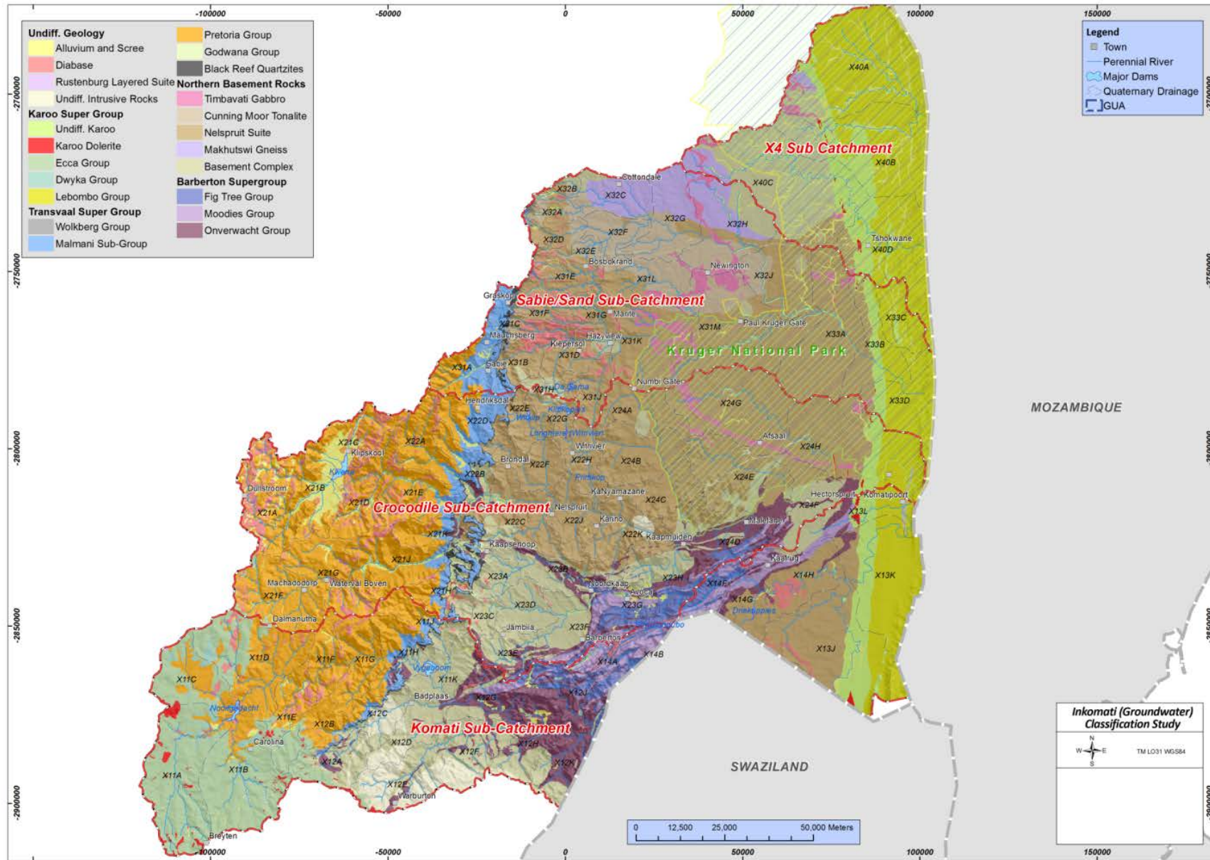
Figure 3.1 Simplified geology of the Inkomati WMA (showing the 4 secondary drainage regions).
