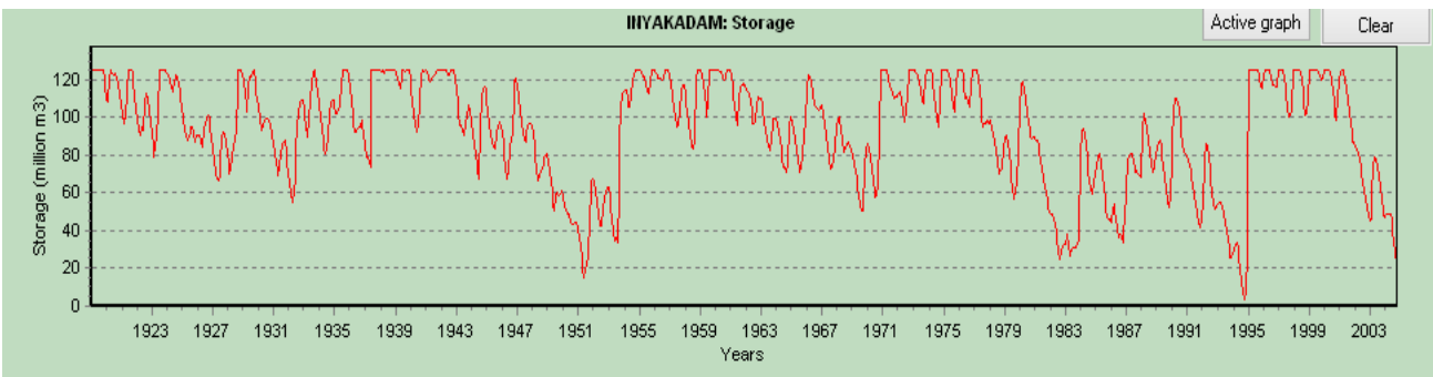
Figure 10.6 Storage in the Inyaka Dam under the Present Day scenario
