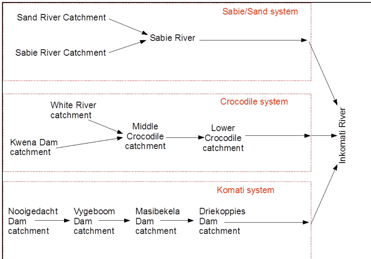
Figure 10.12 Schematic network for the Komati River system
