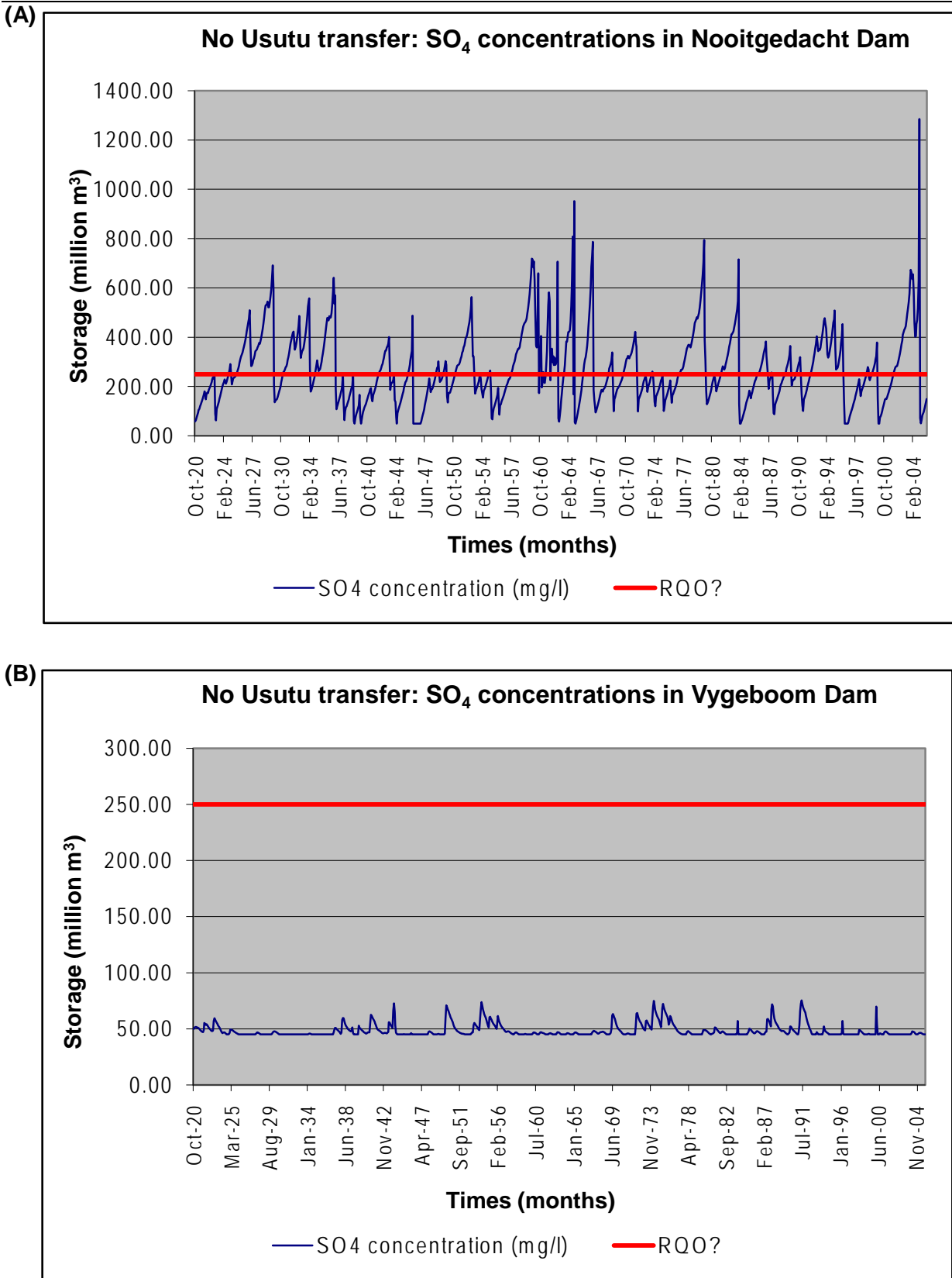
Figure 12.9 Results of the scenario WITH NO TRANSFERS FROM USUTHU for Nooitgedacht (A) and Vygeboom (B) dams
