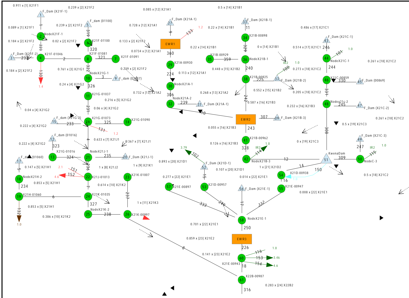
Figure 10.17 Systems diagram of the Upper Crocodile and Elands catchments
