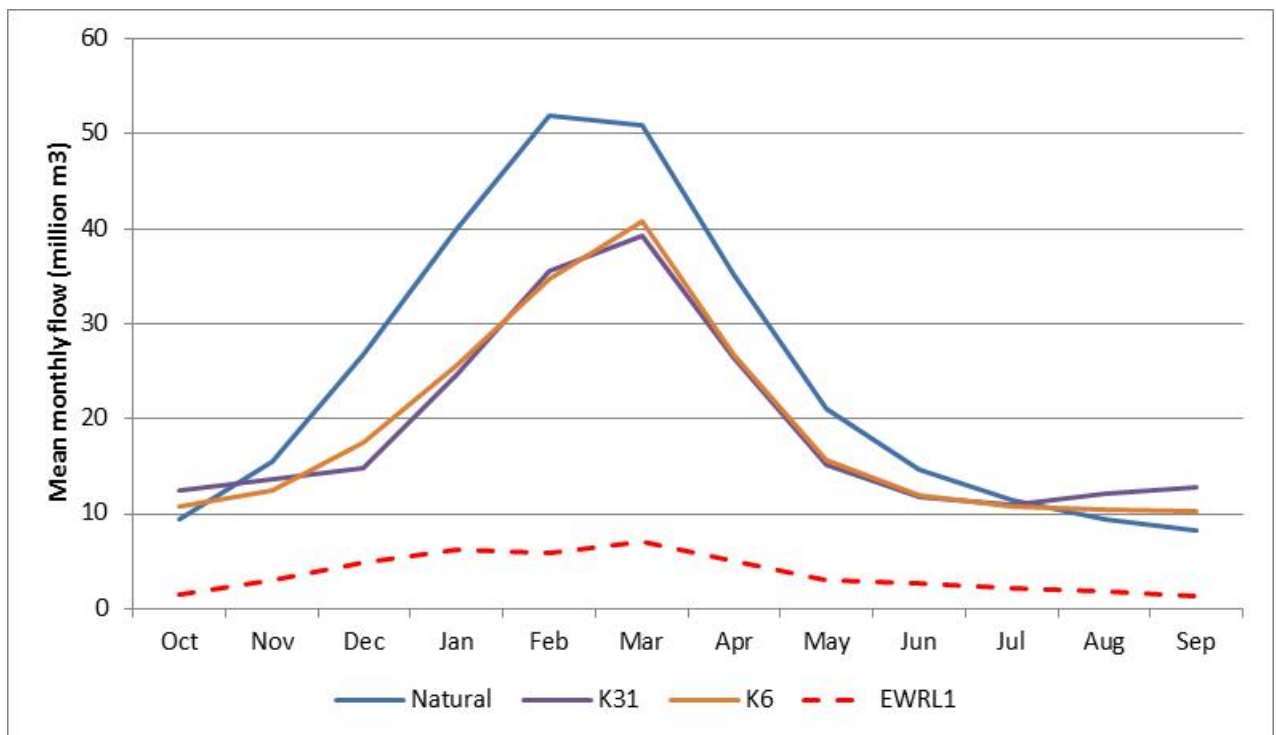
Figure 10.8 Lomati River: Average monthly flows at EWR L1 for selected scenarios
