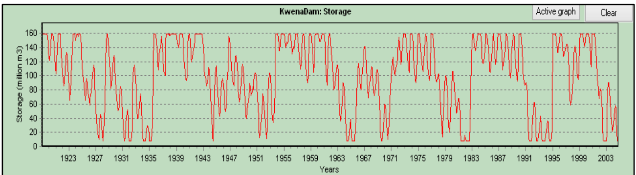
Figure 10.5 Storage in the Kwena Dam under the Present Day scenario
