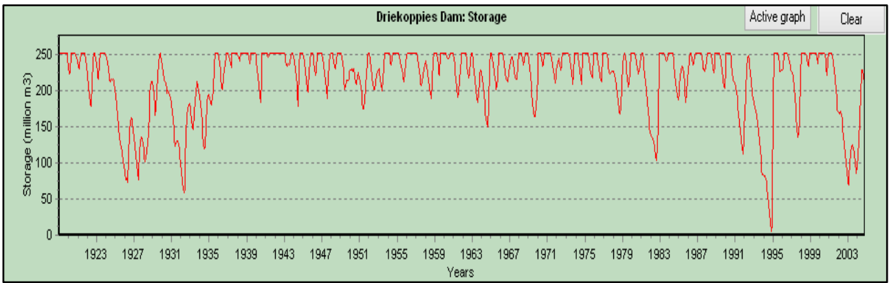
Figure 10.4 Storage in the Driekoppies Dam under the Present Day scenario
