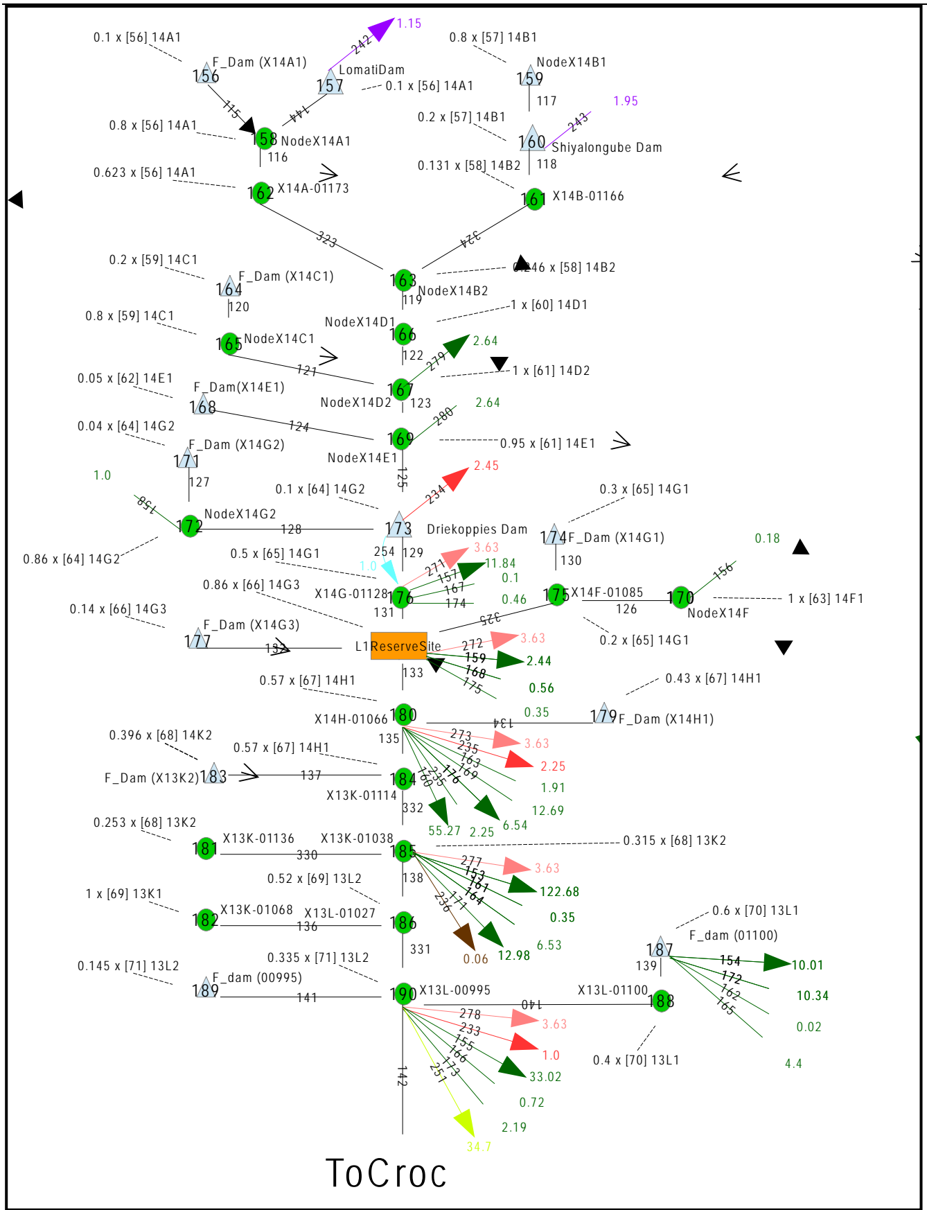
Figure 10.16 Systems diagram of the Lomati and lower Komati
