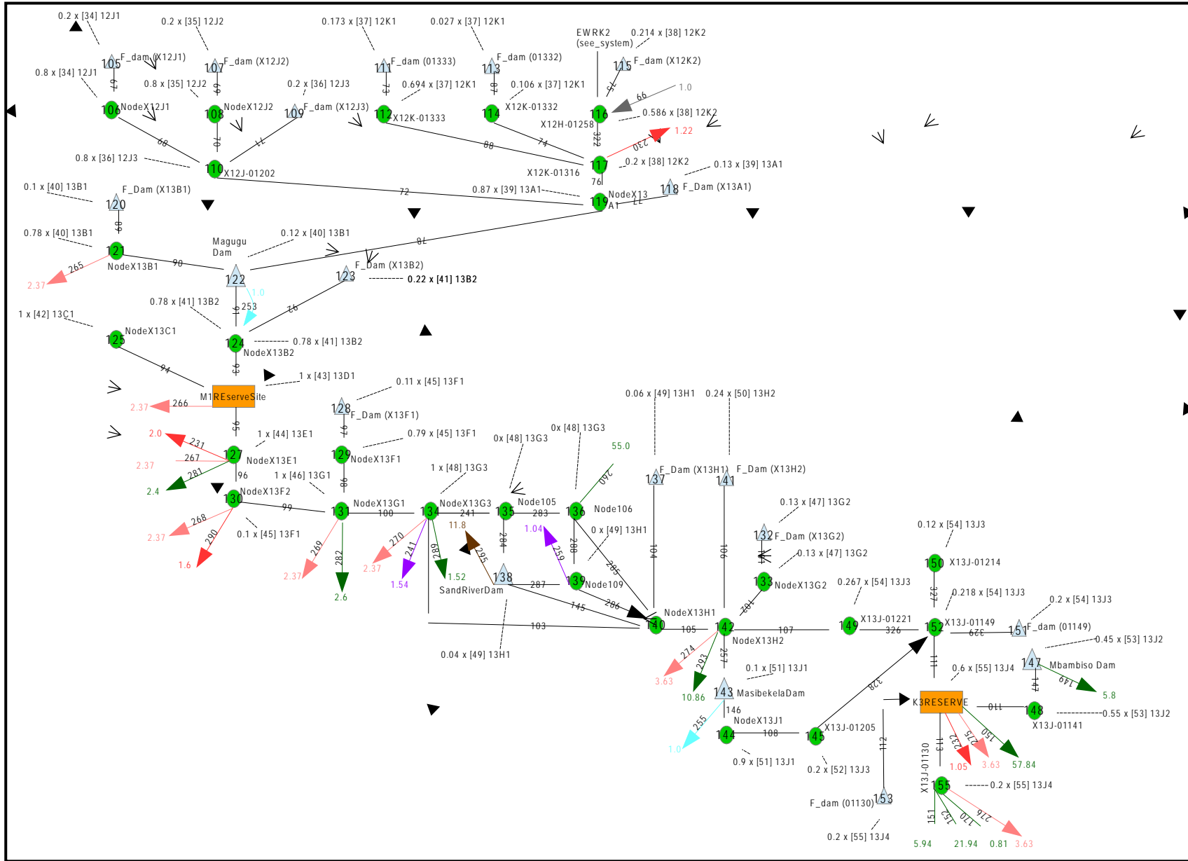
Figure 10.15 Systems diagram of the Middle Komati
