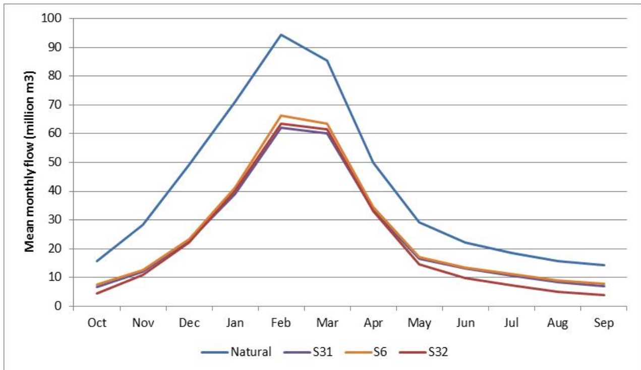
Figure 10.10 Sabie River: Average monthly flows at EWR 3 for selected scenarios
