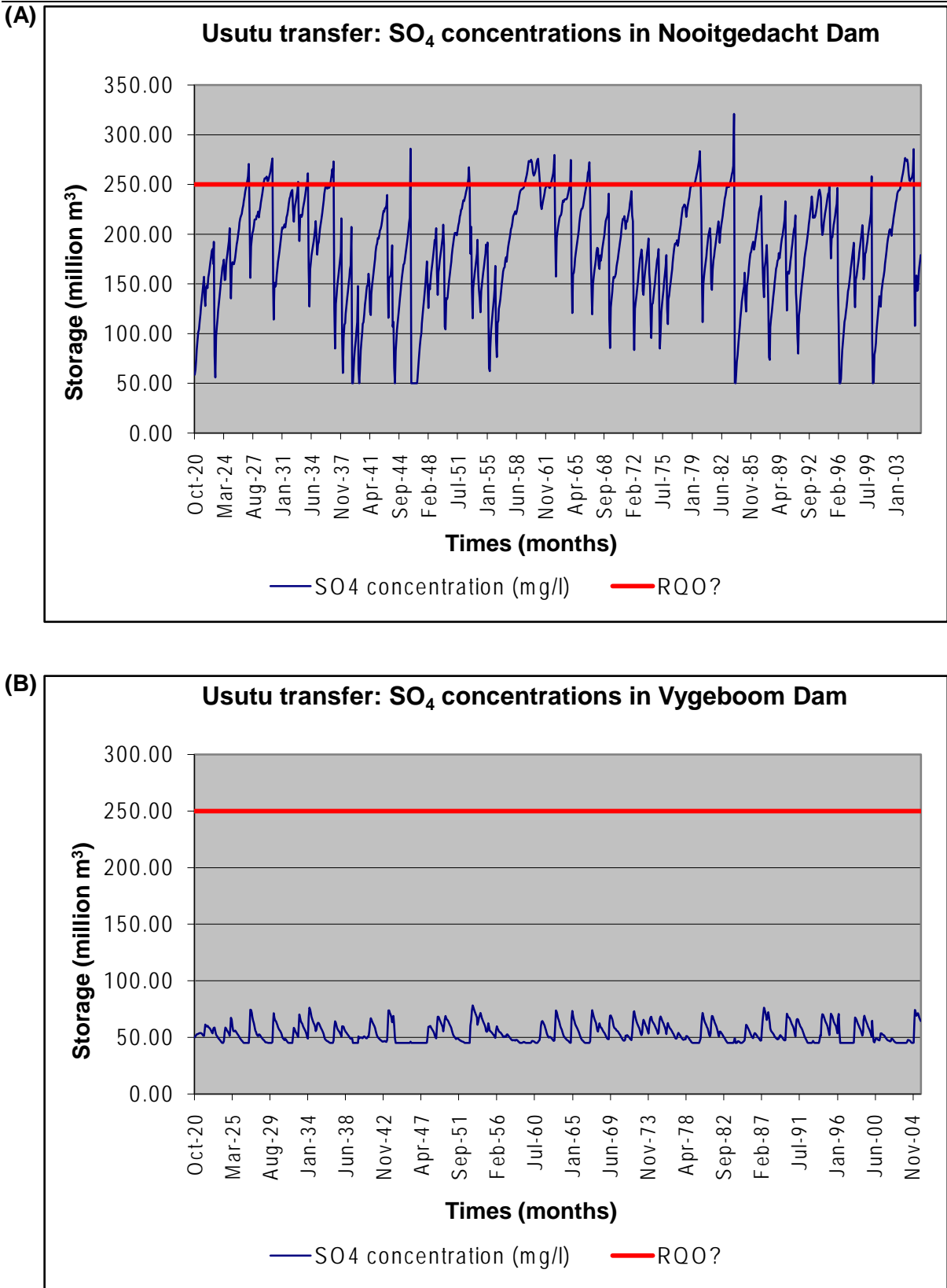
Figure 12.8 Results of the scenario WITH TRANSFERS FROM USUTHU for Nooitgedacht (A) and Vygeboom (B) dams
