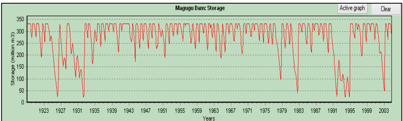
Figure 10.3 Storage in the Maguga Dam under the Present Day scenario
