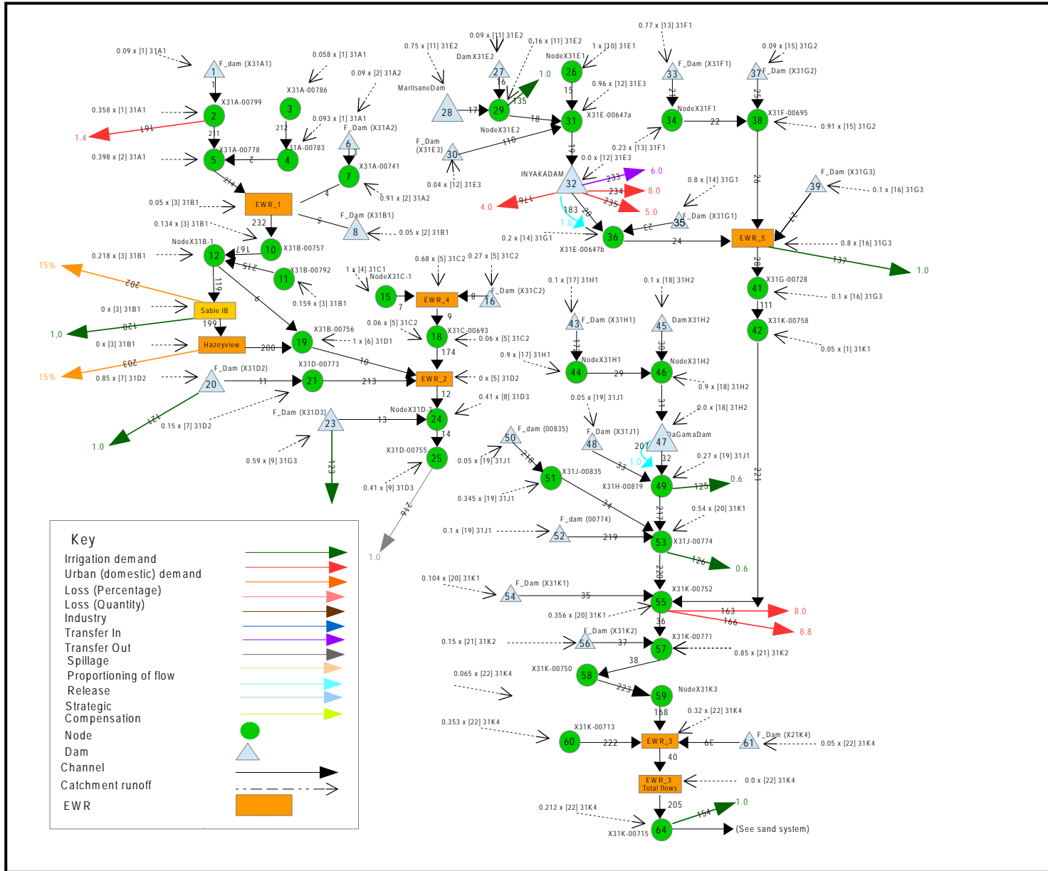
Figure 10.21 Systems diagram of the Sabie River system
