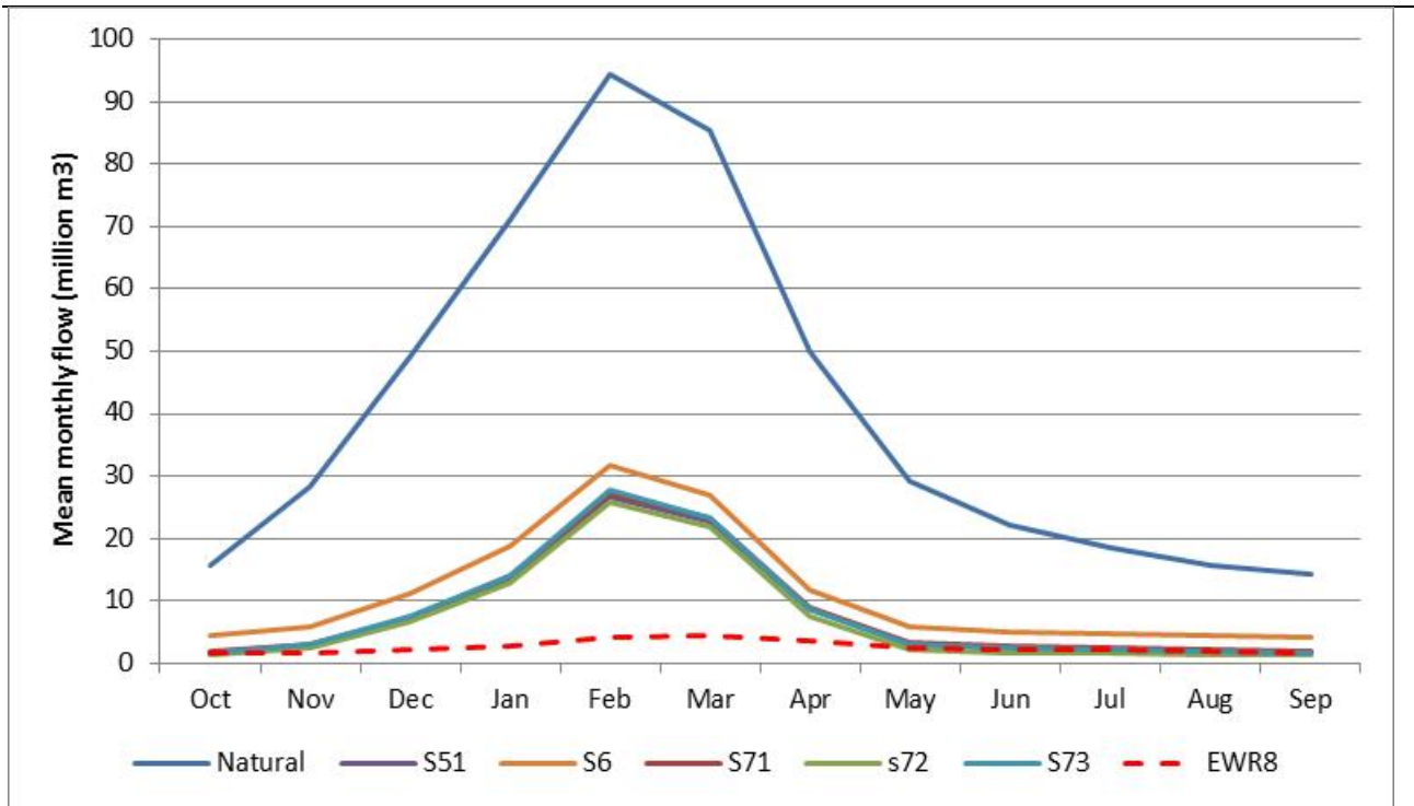
Figure 10.11 Sand River: Average monthly flows at EWR8 for selected scenarios
