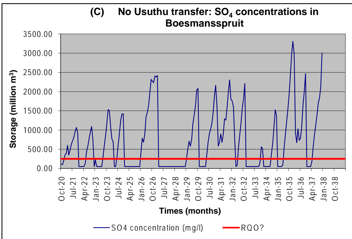
Figure 10.9 Results of the scenario WITH NO TRANSFERS FROM USUTHU for Nooitgedacht (A), Vygeboom (B) and Boesmanspruit (C) dams
