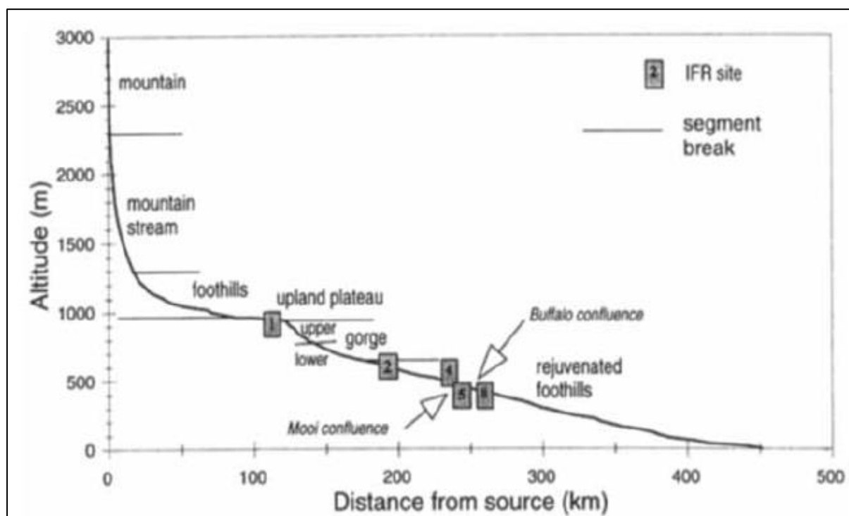
Figure 9: Longitudinal profile of the Thukela River (after Rowntree and Wadeson, 1998)
