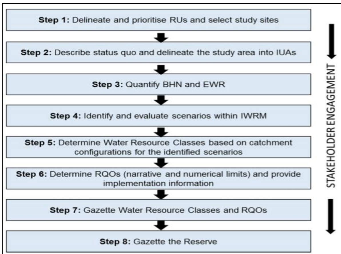
Figure 2: Water resource classes and RQOs determination in the Thukela catchment (integrated process in adherence to Regulation 810 of Government Gazette 33541)
