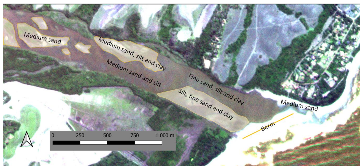
Figure 18: A map of the main sediment types in the Thukela Estuary in September 2020
