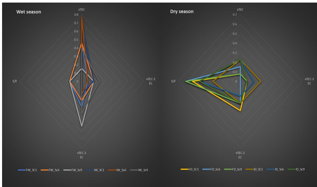
Figure 6: Radar diagram of the ecological consequences outcomes
