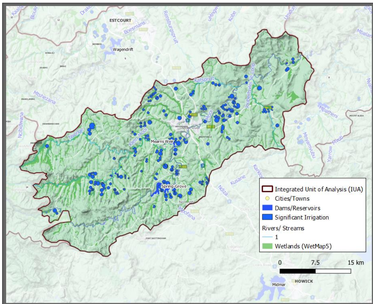
Figure 26: Locality of the demands, and ecological infrastructure are indicated for IUA 7
