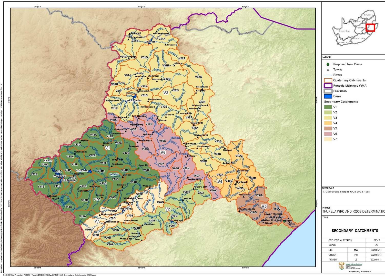
Figure 1: Secondary catchment area boundaries within the Thukela (V1 to V7)
