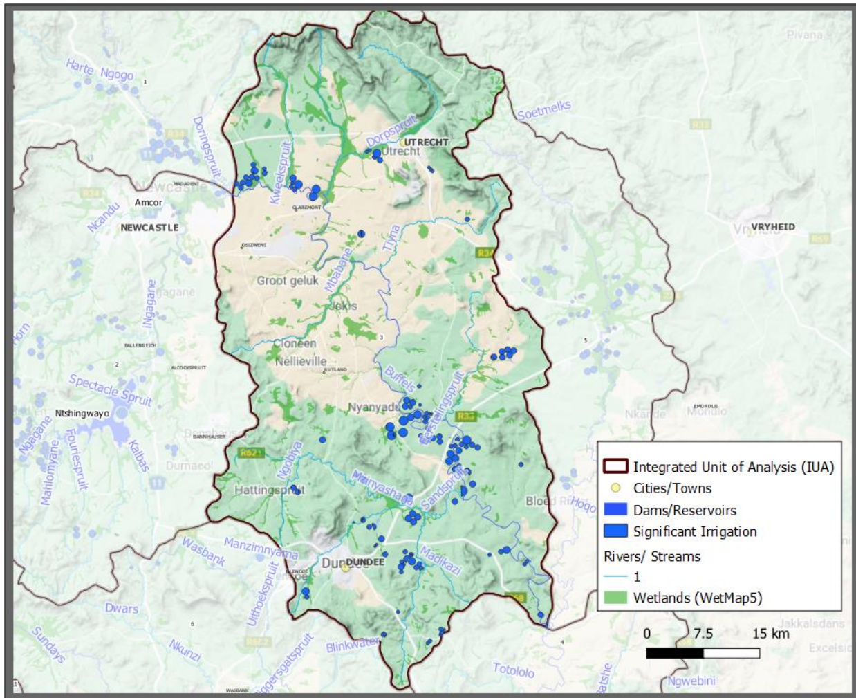
Figure 22: Locality of the demands, and ecological infrastructure are indicated for IUA 3
