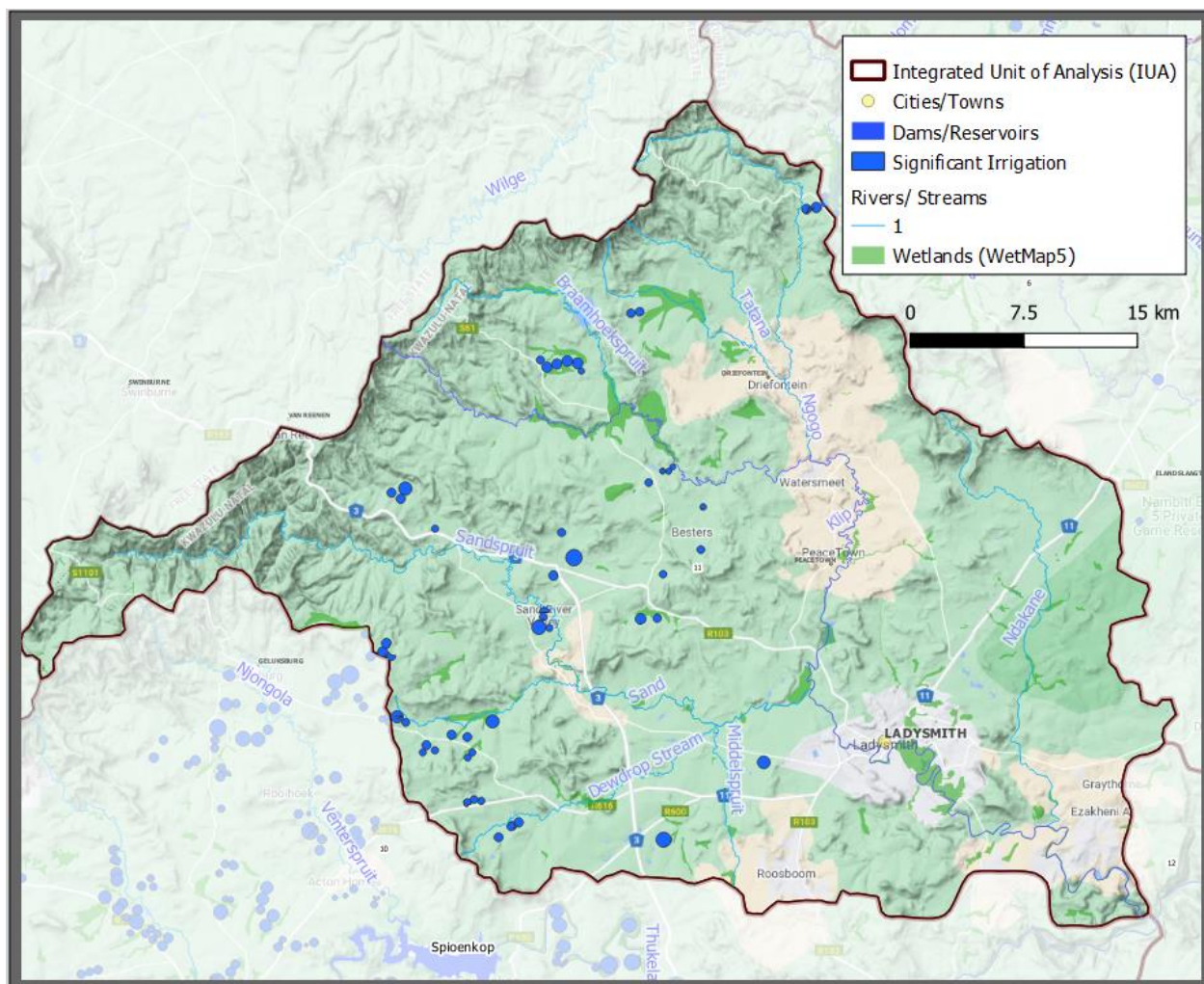
Figure 30: Locality of the demands, and ecological infrastructure are indicated for IUA 11
