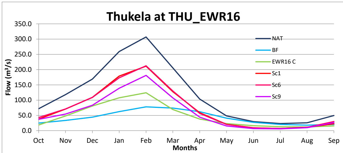
IUA13, Seasonal distribution graph for various flow scenarios at key site THU_EWR16
