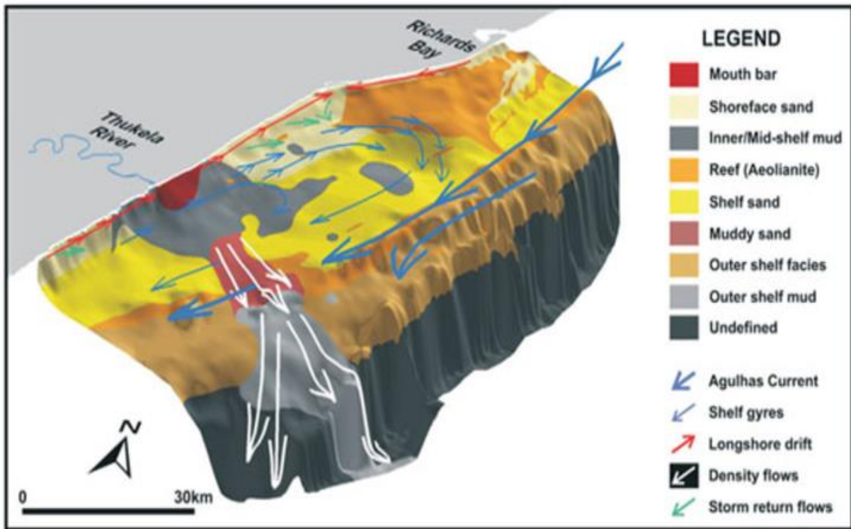
Figure 11: Representation of the Thukela banks (Image by Bosman et al., 2007)
