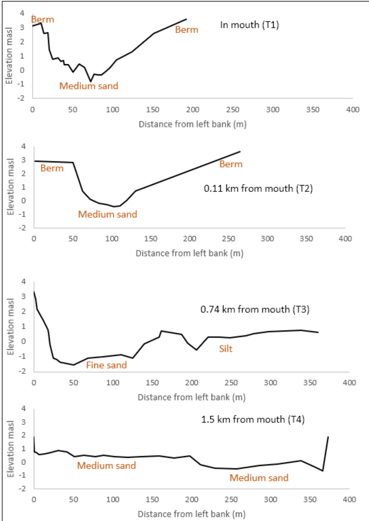
Figure 15: Cross sectional surveys of the Thukela Estuary
