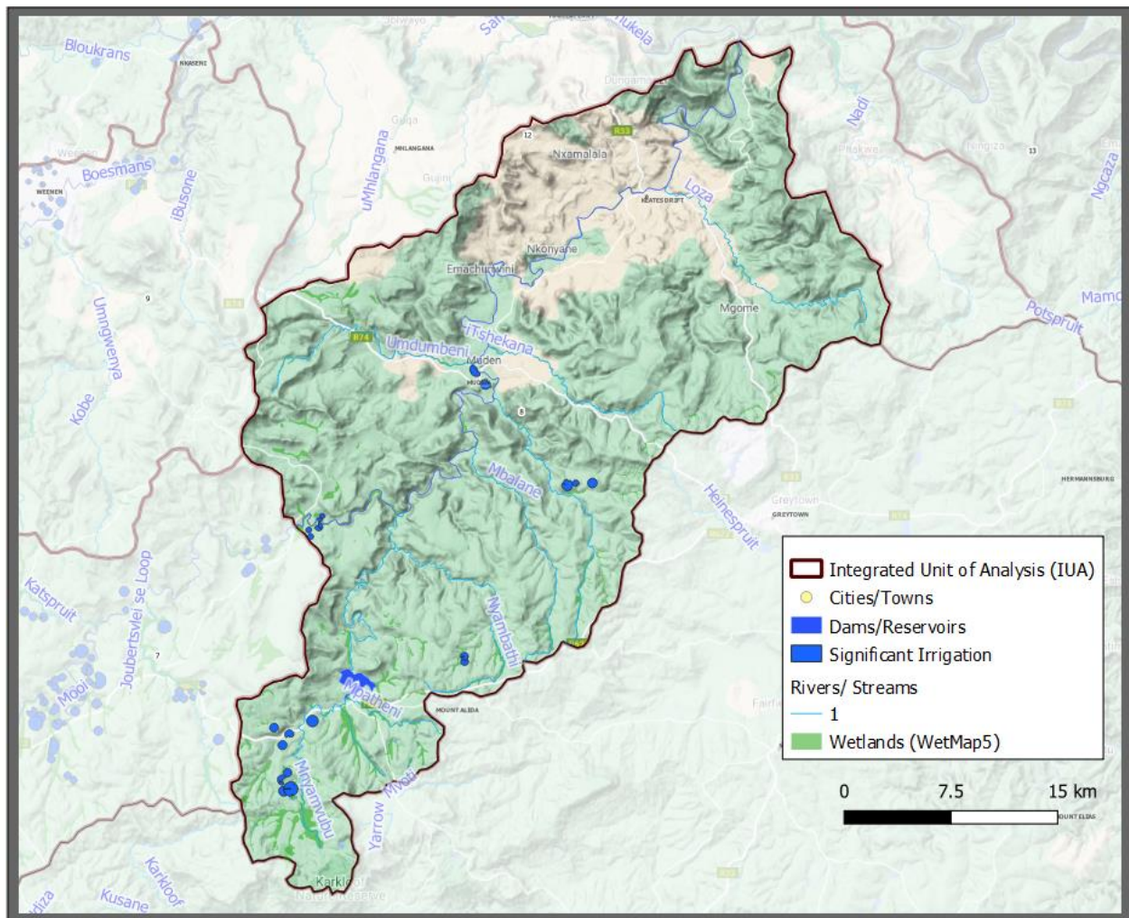
Figure 27: Locality of the demands, and ecological infrastructure are indicated for IUA 8
