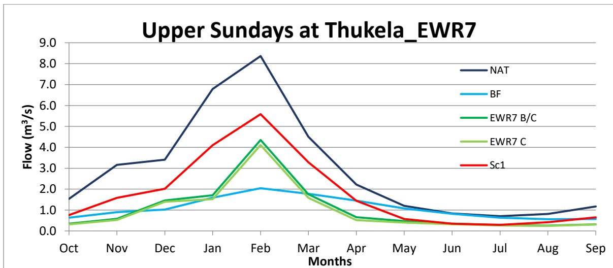
IUA6, Seasonal distribution graph for various flow scenarios at key site Thukela_EWR7
