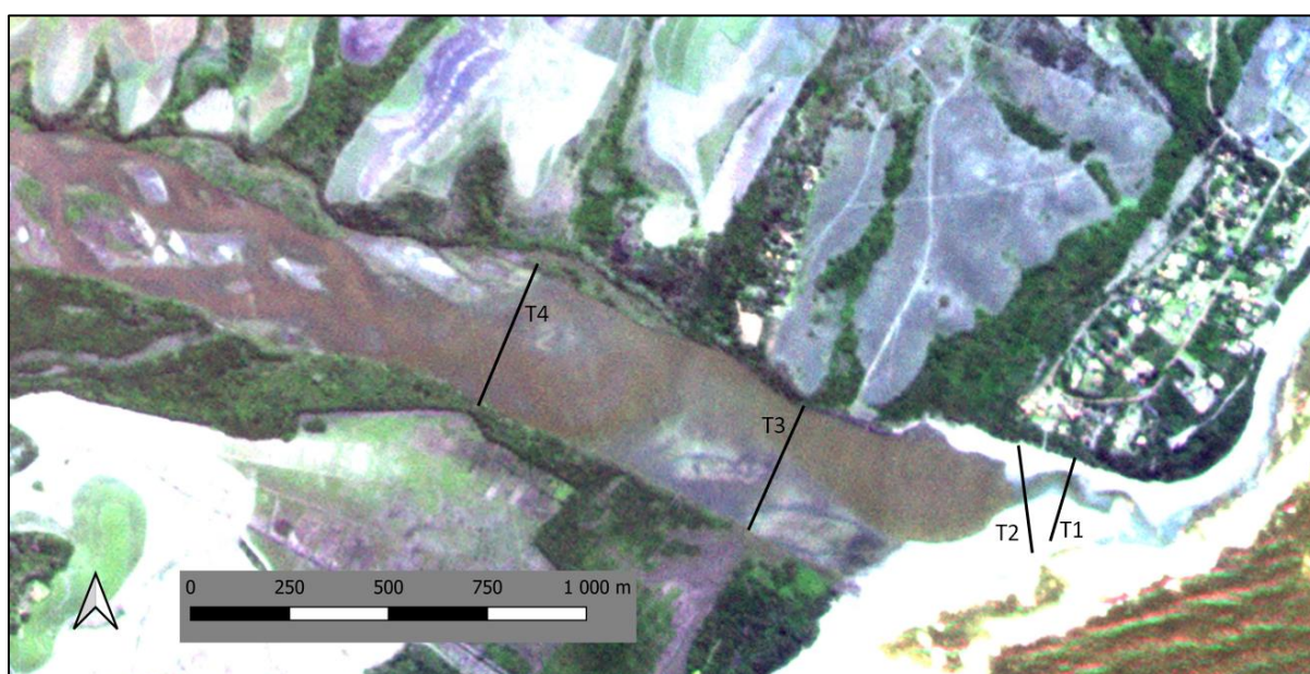
Figure 13: Location of the transects 1 to 4. Satellite image captured at 9am, 17 September 2020 at low tide and coincides with the cross-section survey date
