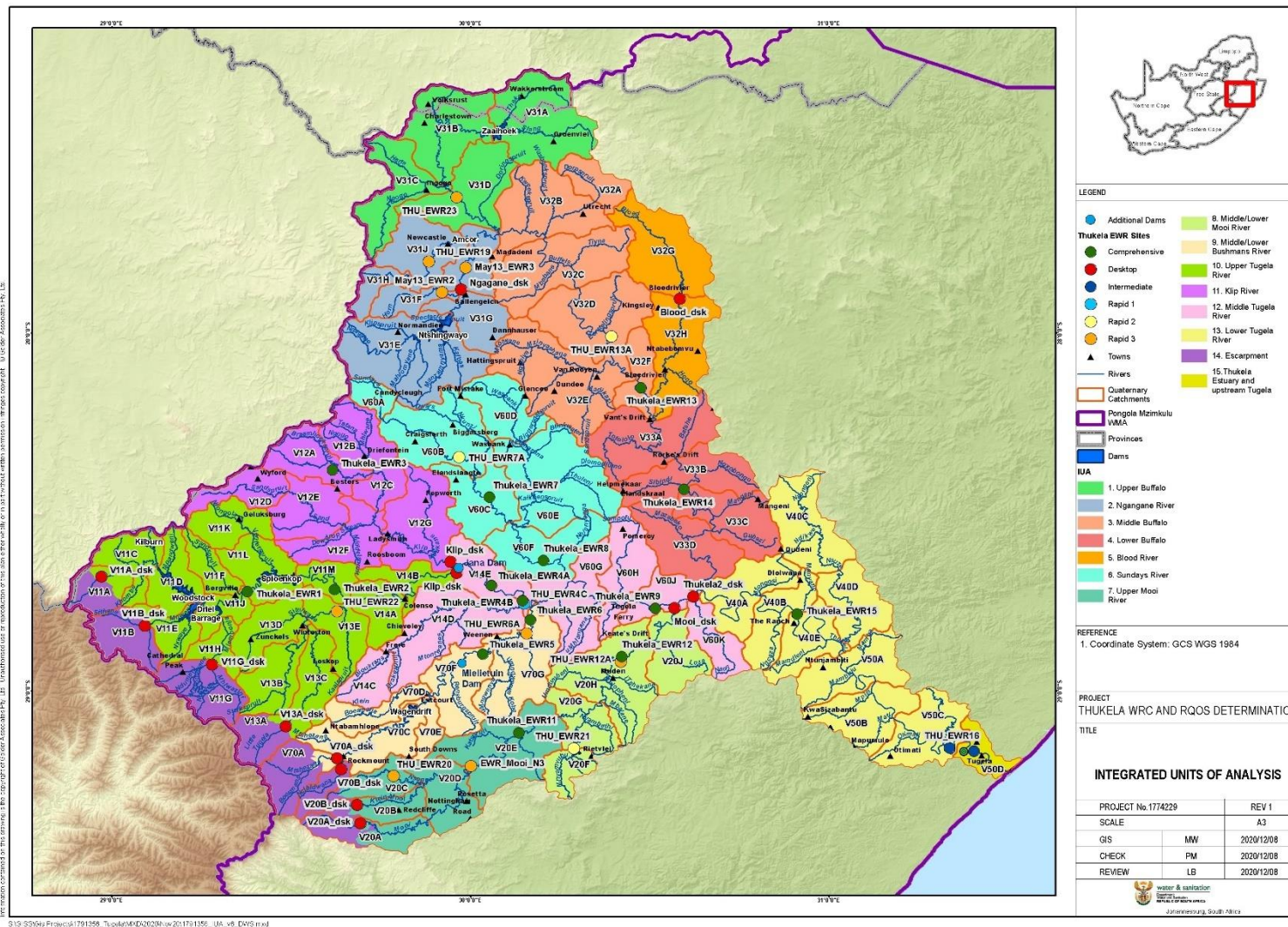
Figure 4: Thukela IUAs with EWR sites and hydronodes
