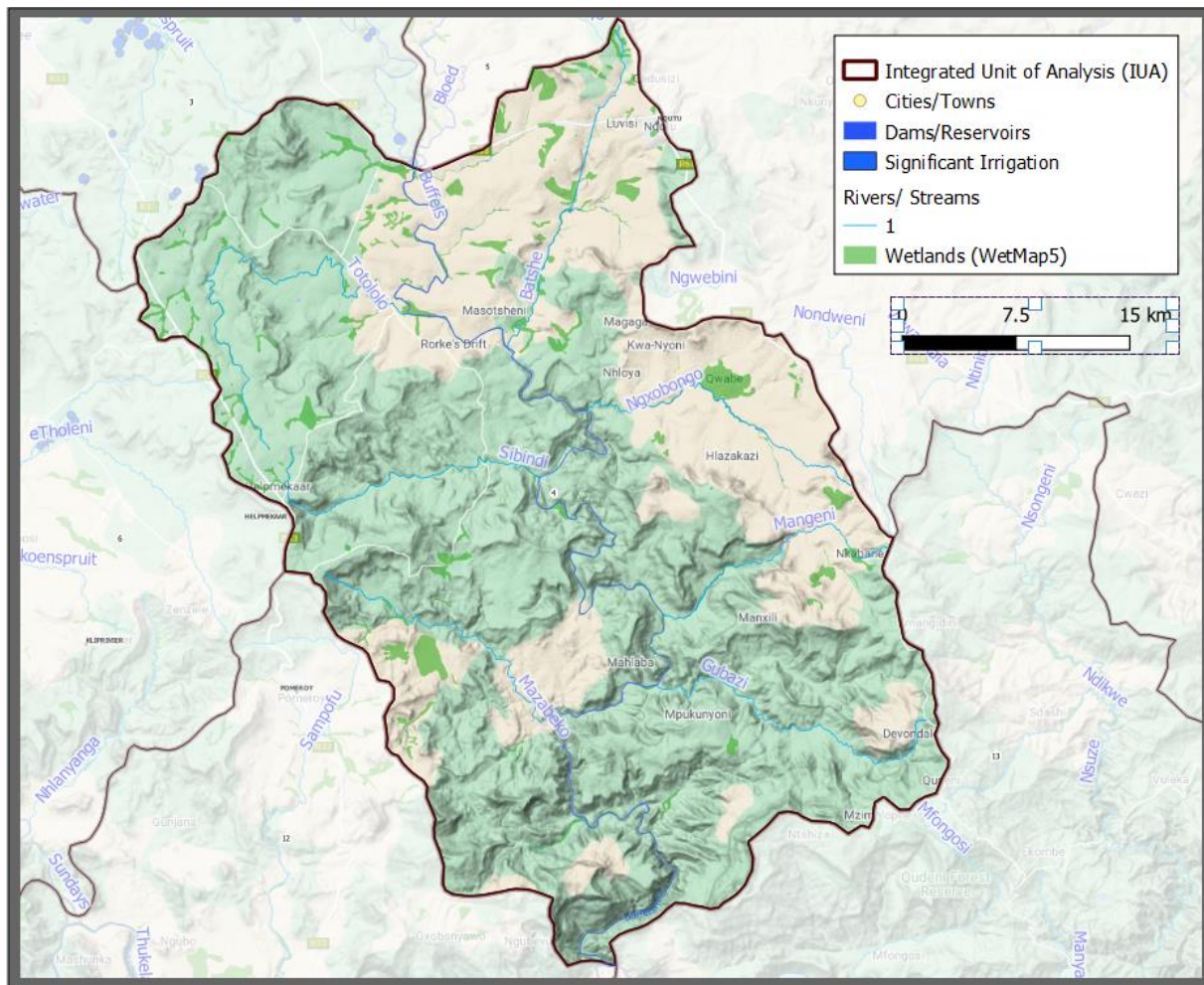
Figure 23: Locality of the demands, and ecological infrastructure are indicated for IUA 4
