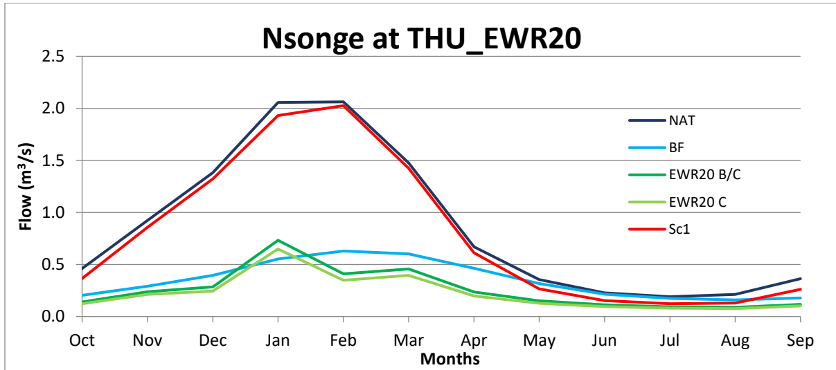
IUA7, Seasonal distribution graph for various flow scenarios at key site THU_EWR20
