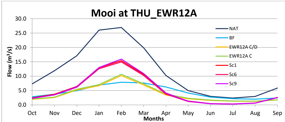
IUA8, Seasonal distribution graph for various flow scenarios at key site THU_EWR12A
