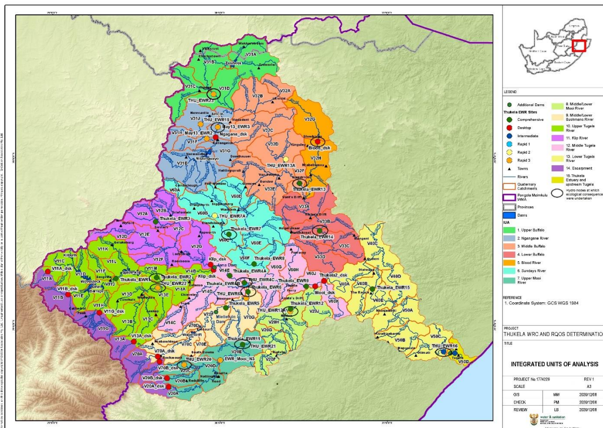
Figure 5: Hydro node sites at which ecological consequences were assessed
