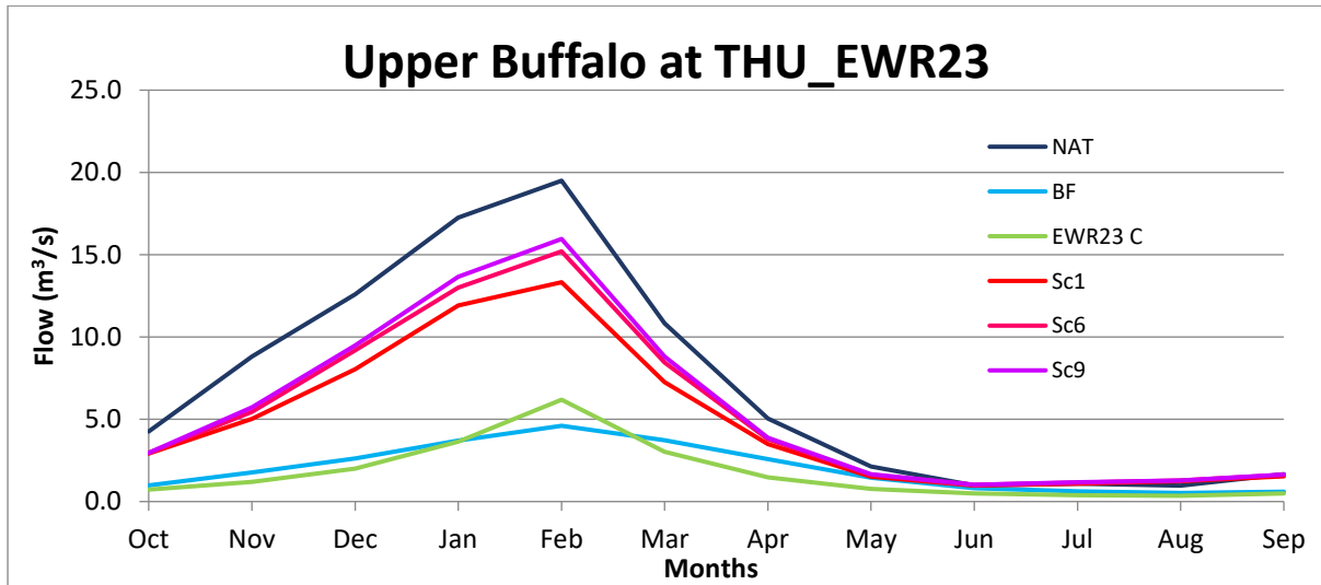
IUA1, Seasonal distribution graph for various flow scenarios at key site THU_EWR23
