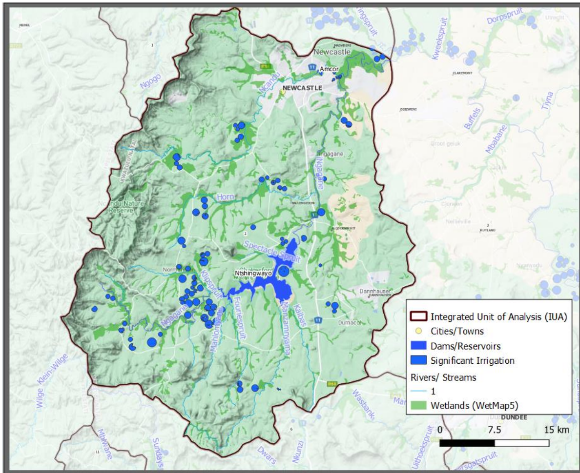
Figure 21: Locality of the demands, and ecological infrastructure are indicated for IUA 2
