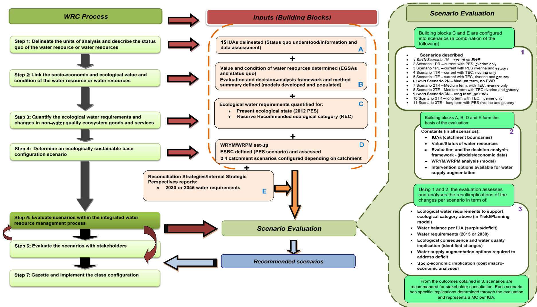
Figure 3: Scenarios evaluation within the integrated water resource management systems
