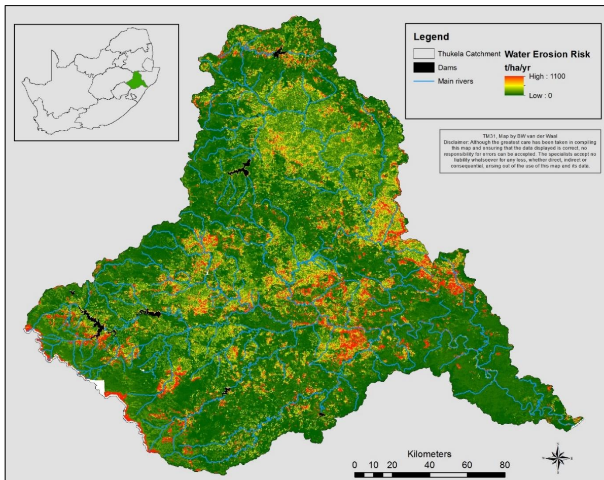
Figure 10: Water erosion potential for the Thukela River catchment (Le Roux et al., 2008)
