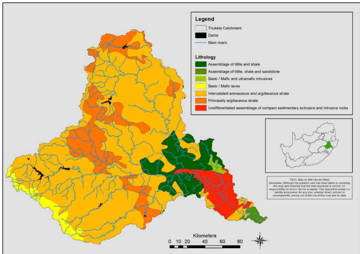
Figure 8: Lithology of the Thukela River basin (Data source: WR90)
