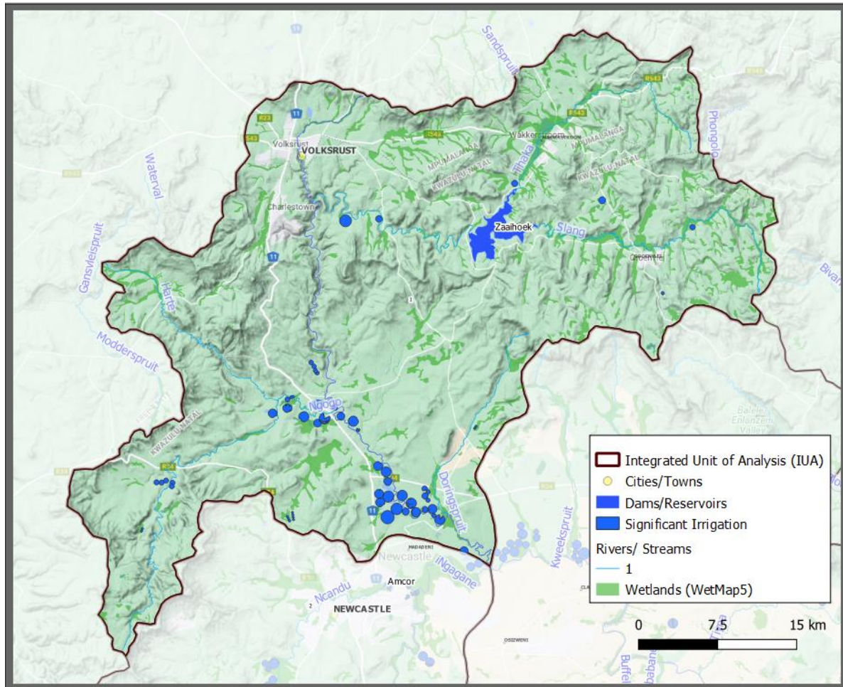
Figure 20: Locality of the demands, and ecological infrastructure are indicated for IUA 1
