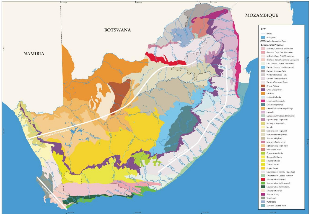
Figure 7: Geomorphic provinces of South Africa (image from Partridge et al., 2010)
