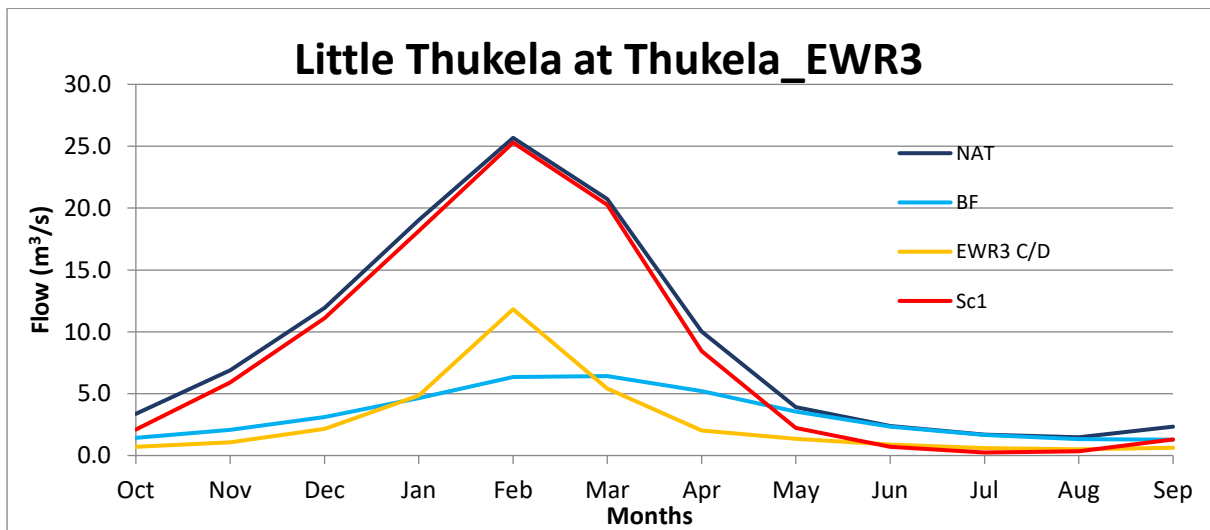
IUA10, Seasonal distribution graph for various flow scenarios at key site Thukela_EWR3
