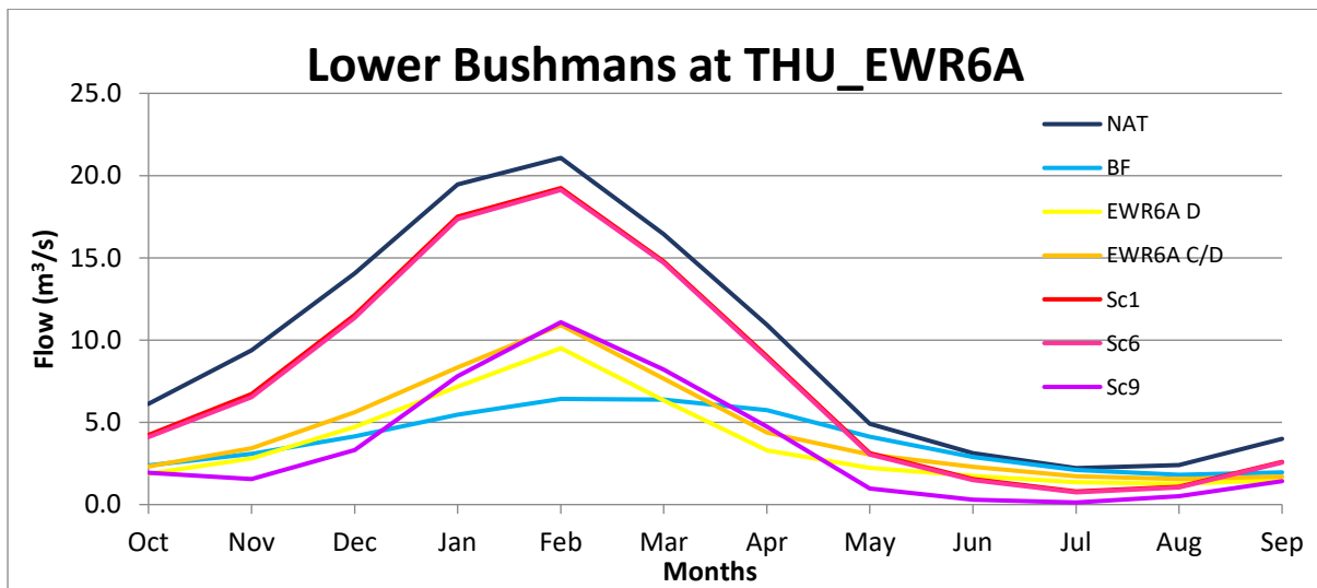
IUA9, Seasonal distribution graph for various flow scenarios at key site THU_EWR6A
