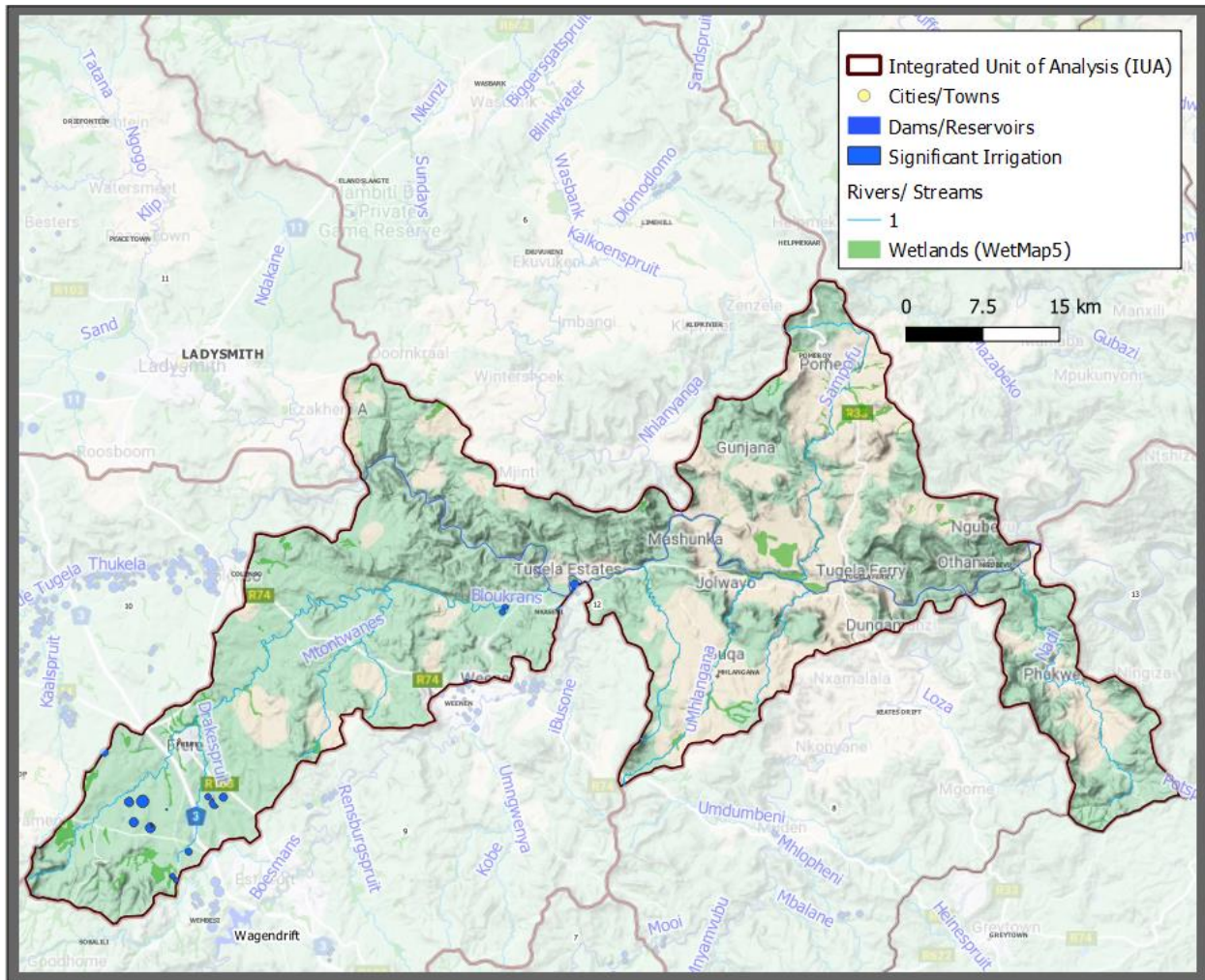
Figure 31: Locality of the demands, and ecological infrastructure are indicated for IUA 12
