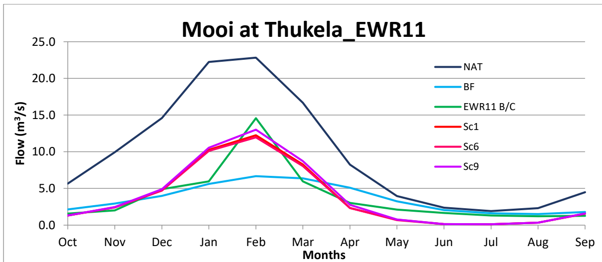
IUA7, Seasonal distribution graph for various flow scenarios at key site Thukela_EWR11
