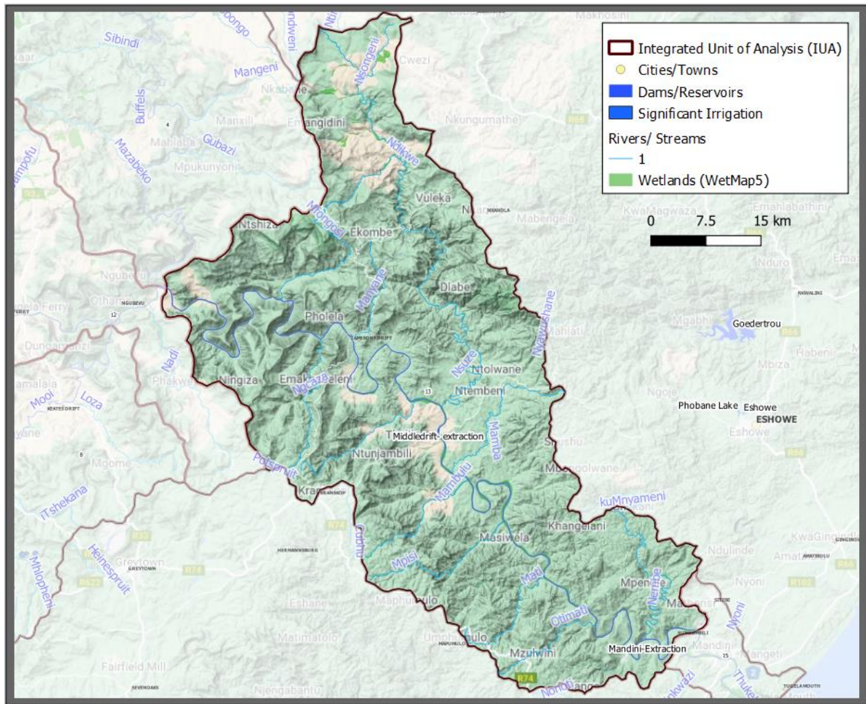
Figure 32: Locality of the demands, and ecological infrastructure are indicated for IUA 13
