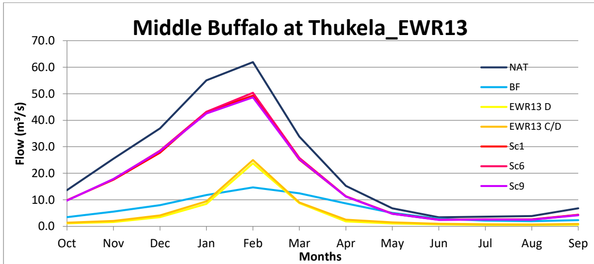
IUA3, Seasonal distribution graph for various flow scenarios at key site Thukela_EWR13
