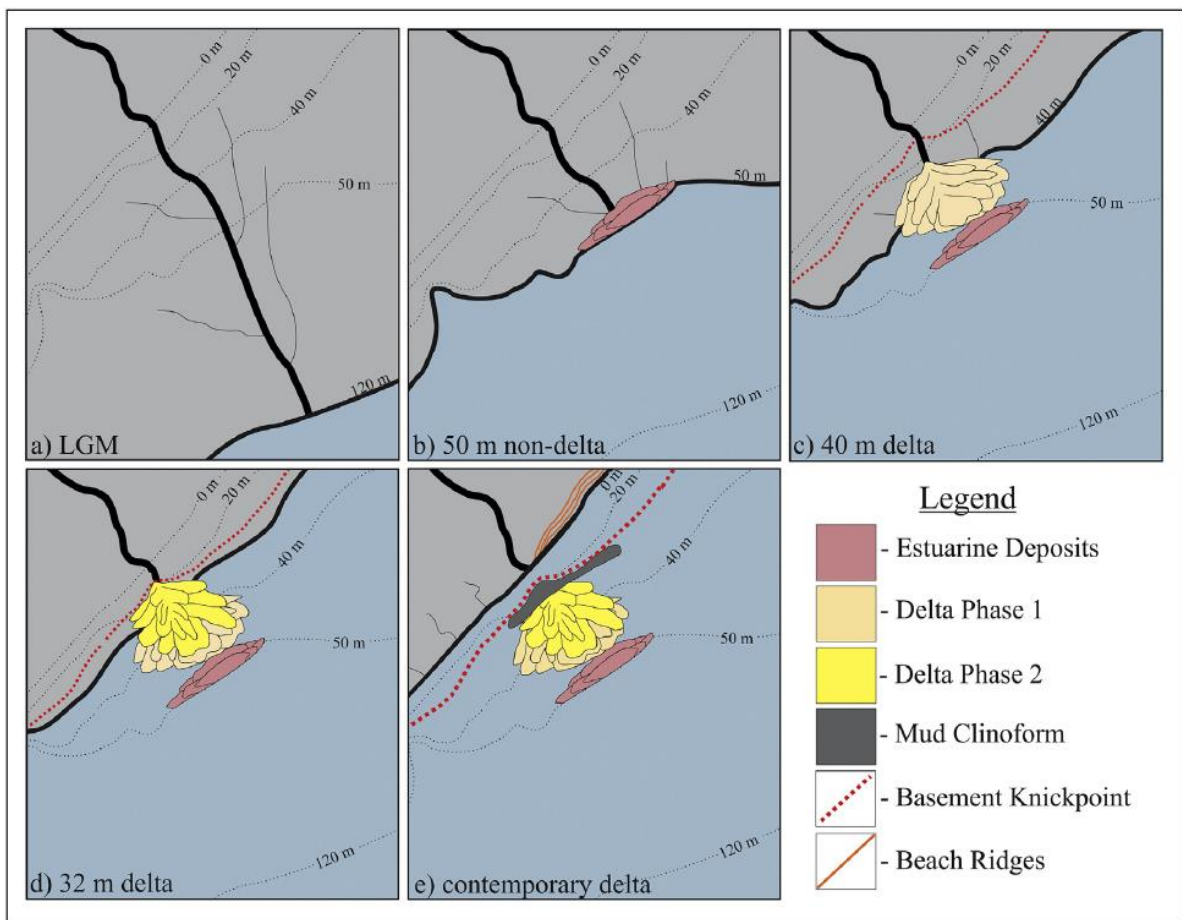
Figure 11: Representation of the Thukela banks (Image by Bosman et al., 2007)
