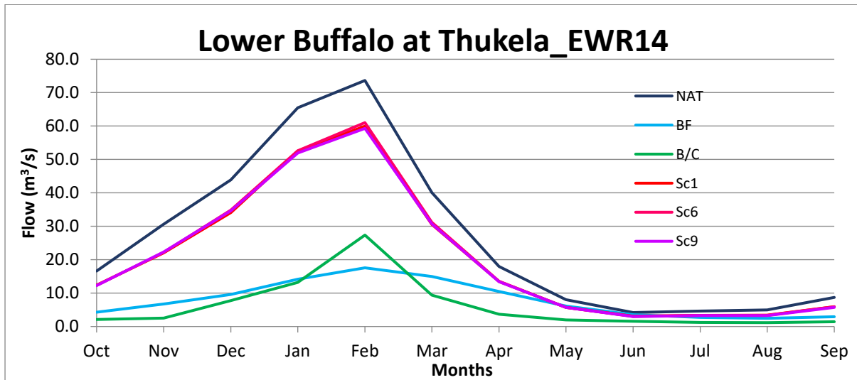
IUA4, Seasonal distribution graph for various flow scenarios at key site Thukela_EWR14
