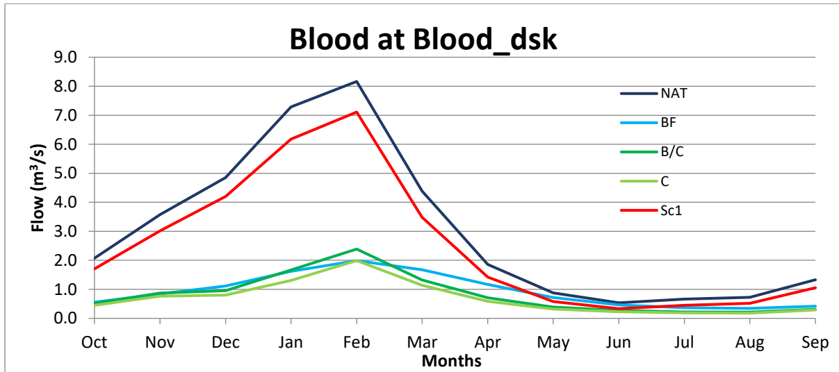
IUA5, Seasonal distribution graph for various flow scenarios at key site Blood_dsk
