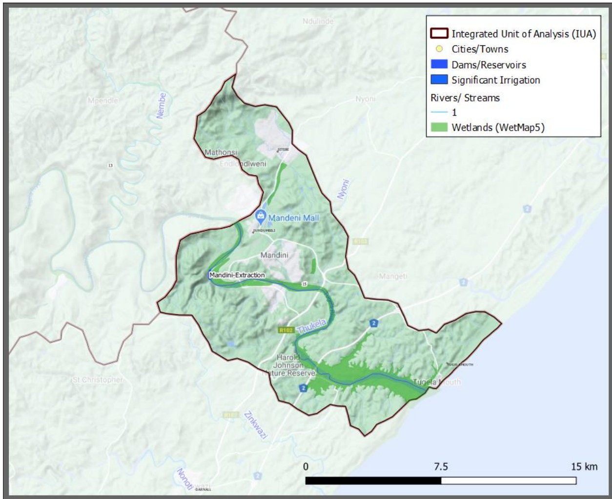
Figure 33: Locality of the demands, and ecological infrastructure are indicated for IUA 15
