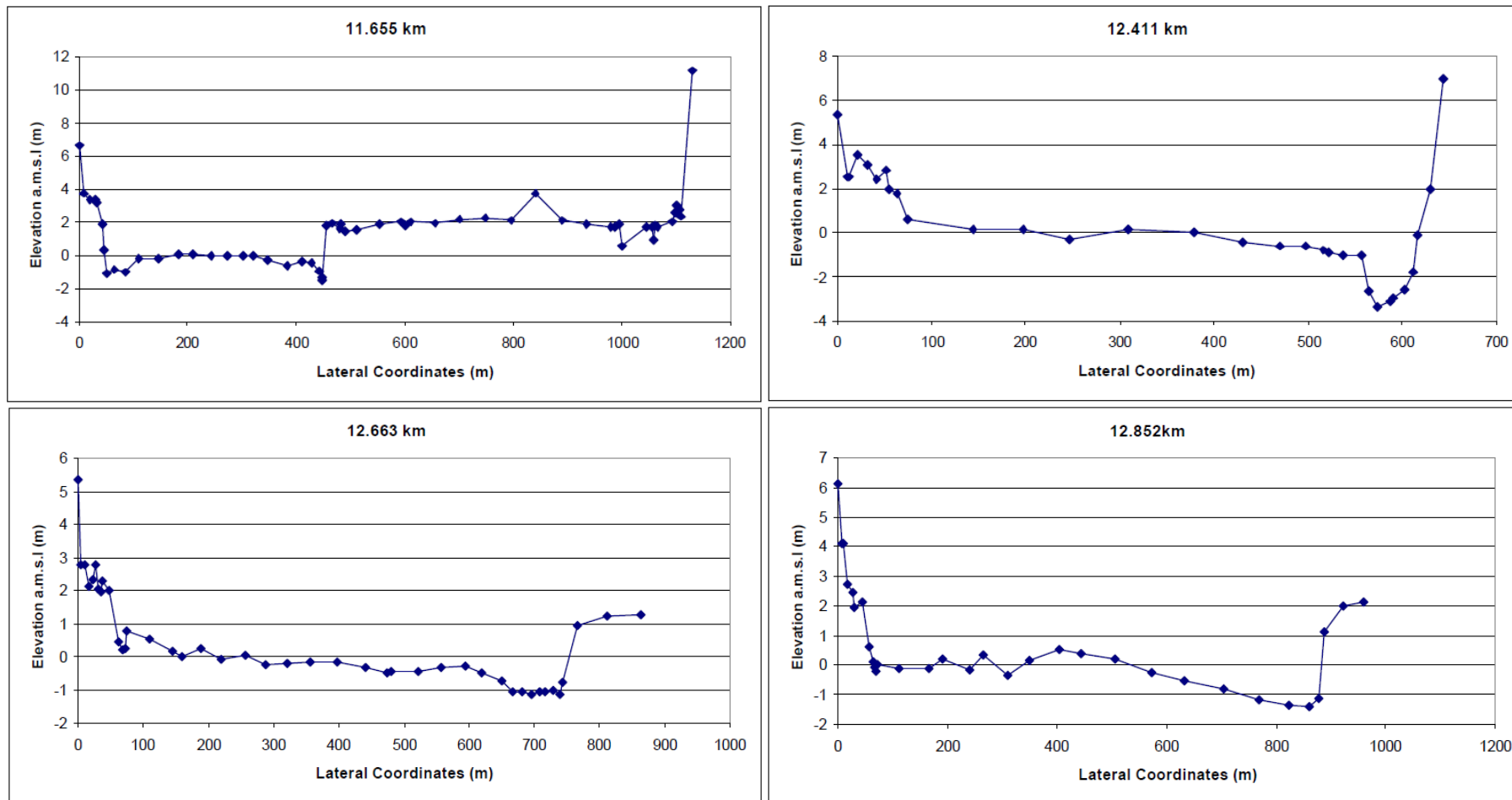
Figure 17: A selection of cross sections from the 1996 survey
