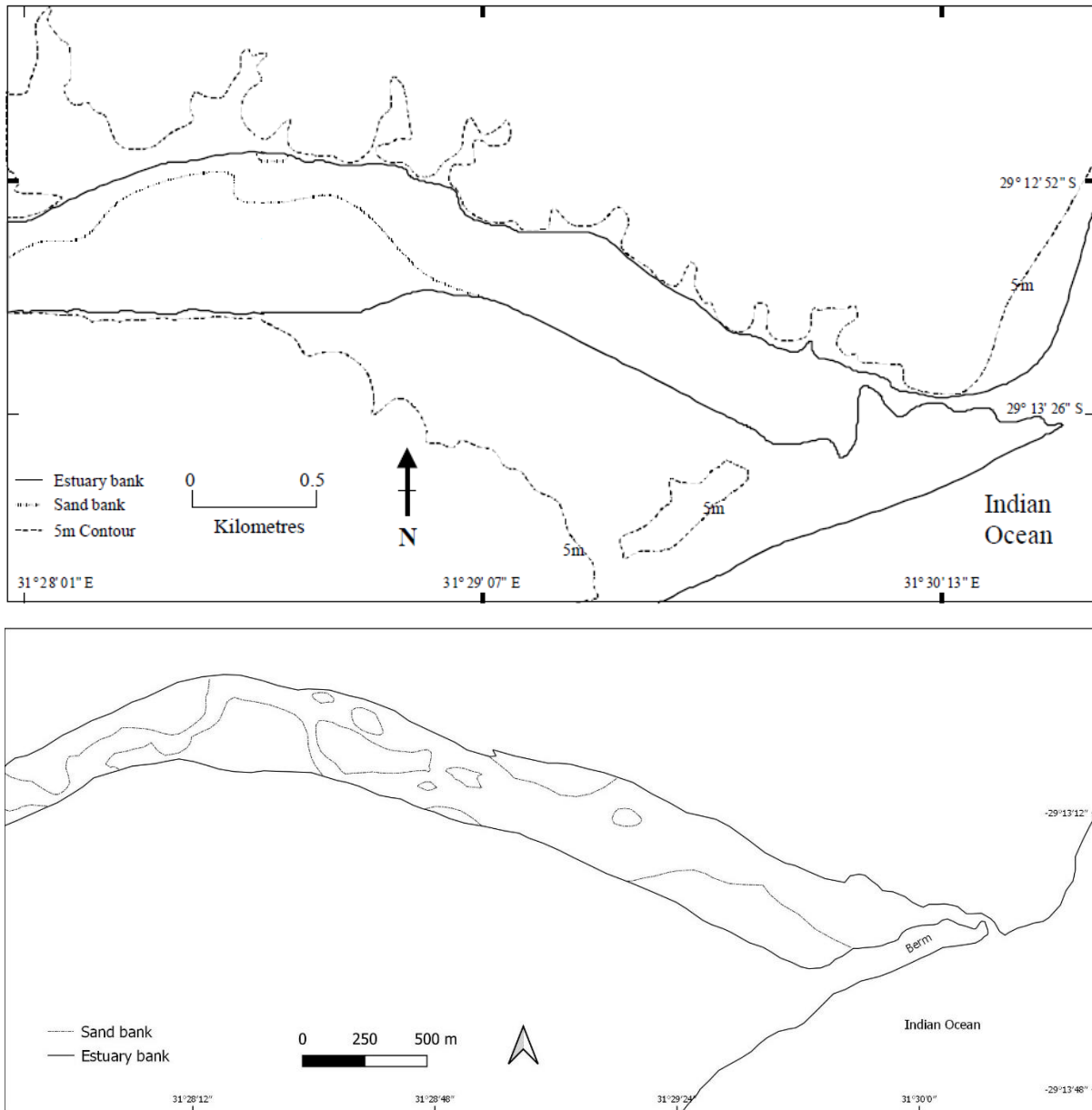
Figure 14: Maps for the Thukela Estuary from: a) 2001 (Taljaard et al., 2004) and b) 17 September 2020 showing the banks of the estuary and the extent of the sand banks
