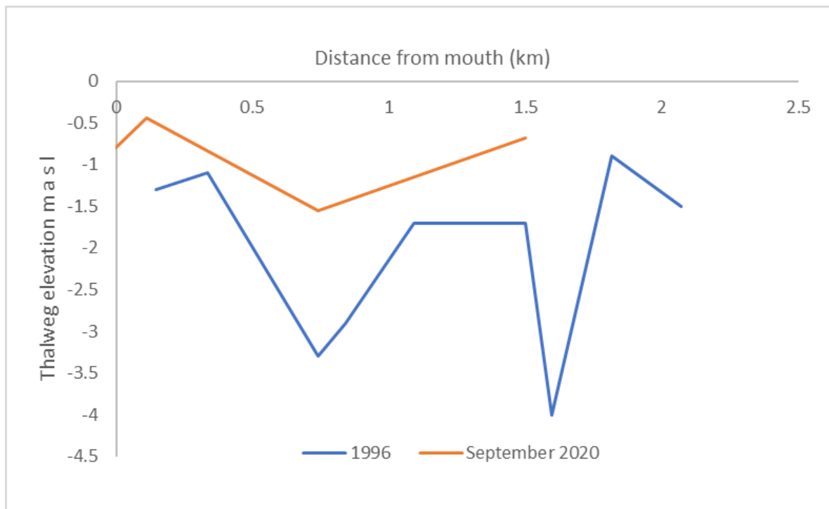
Figure 16: Longitudinal profile of the lower 2 km of the Thukela Estuary showing bed elevation in 1996 and 2020
