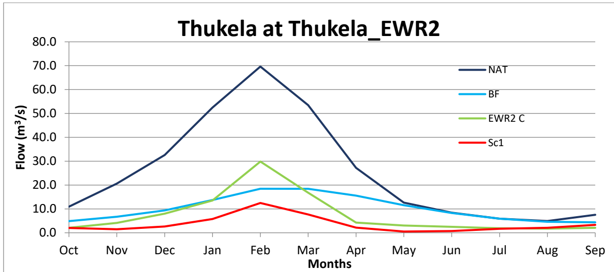
IUA10, Seasonal distribution graph for various flow scenarios at key site Thukela_EWR2
