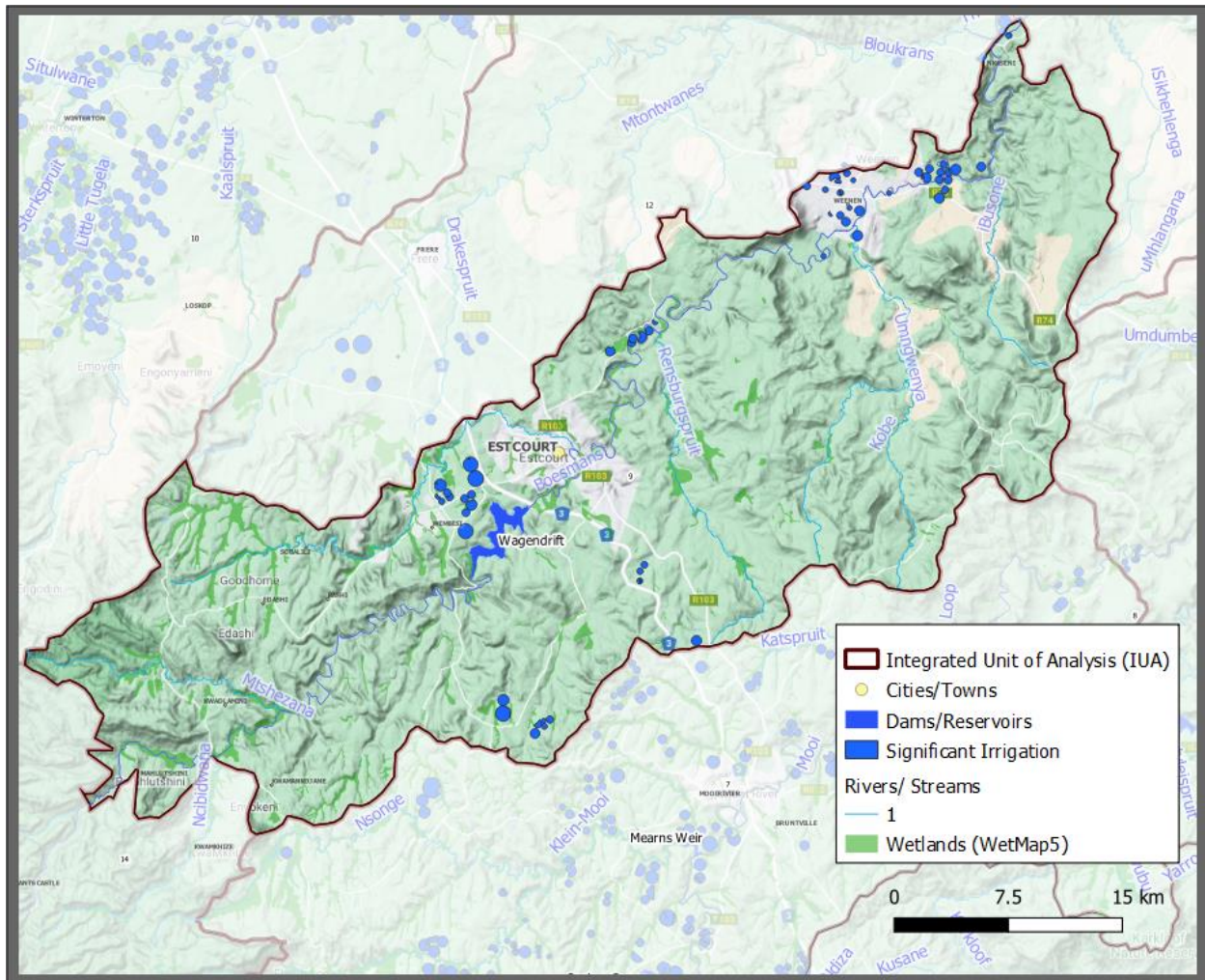
Figure 28: Locality of the demands, and ecological infrastructure are indicated for IUA 9
