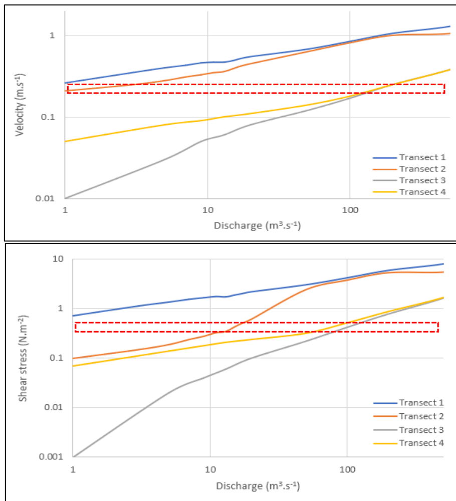
Figure 19: Discharge-velocity and discharge-shear stress curves for Transect 1 to 4 of the Thukela Estuary (The red dashed box indicates the threshold for medium sand entrainment)
