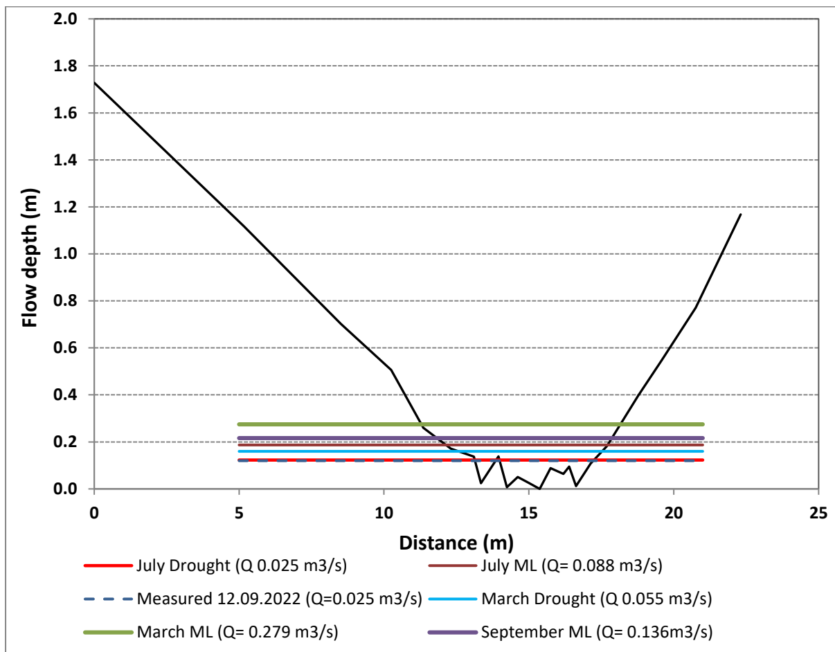
Figure 6-24: Water levels on cross-section of the EWR site for Lower Kat River in Q94F.
