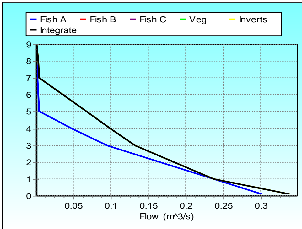
Figure 5-38: Final integrated stress curve for the Upper Kat EWR site (KAT01_I).
