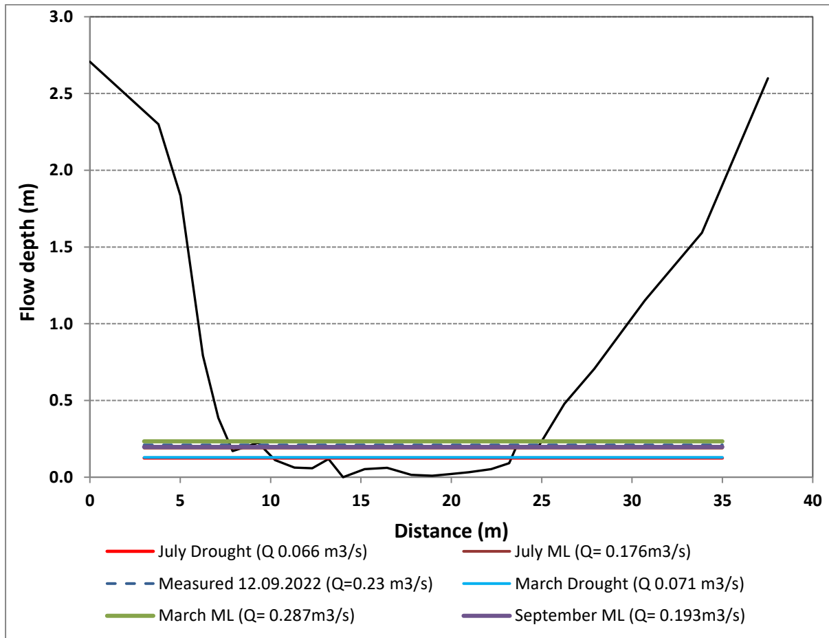
Figure 6-22: Water levels on cross-section of the EWR site for Koonap River in Q92G.
