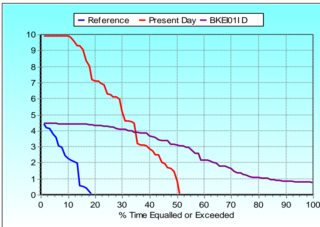
Figure 5-15: Final stress duration curves – wet season (March).
