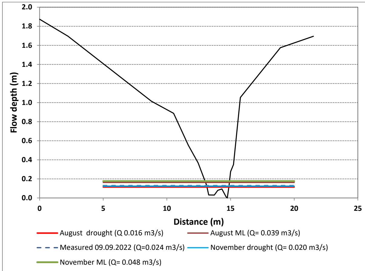
Figure 6-4: Water levels on cross-section of the EWR site for Nqabara River in T90A.
