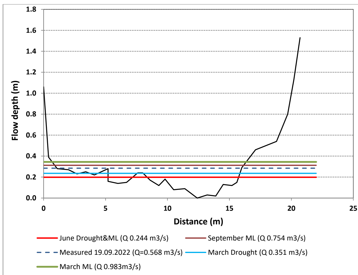
Figure 6-18: Water levels on cross-section of the EWR site for Keiskamma River in R10L.
