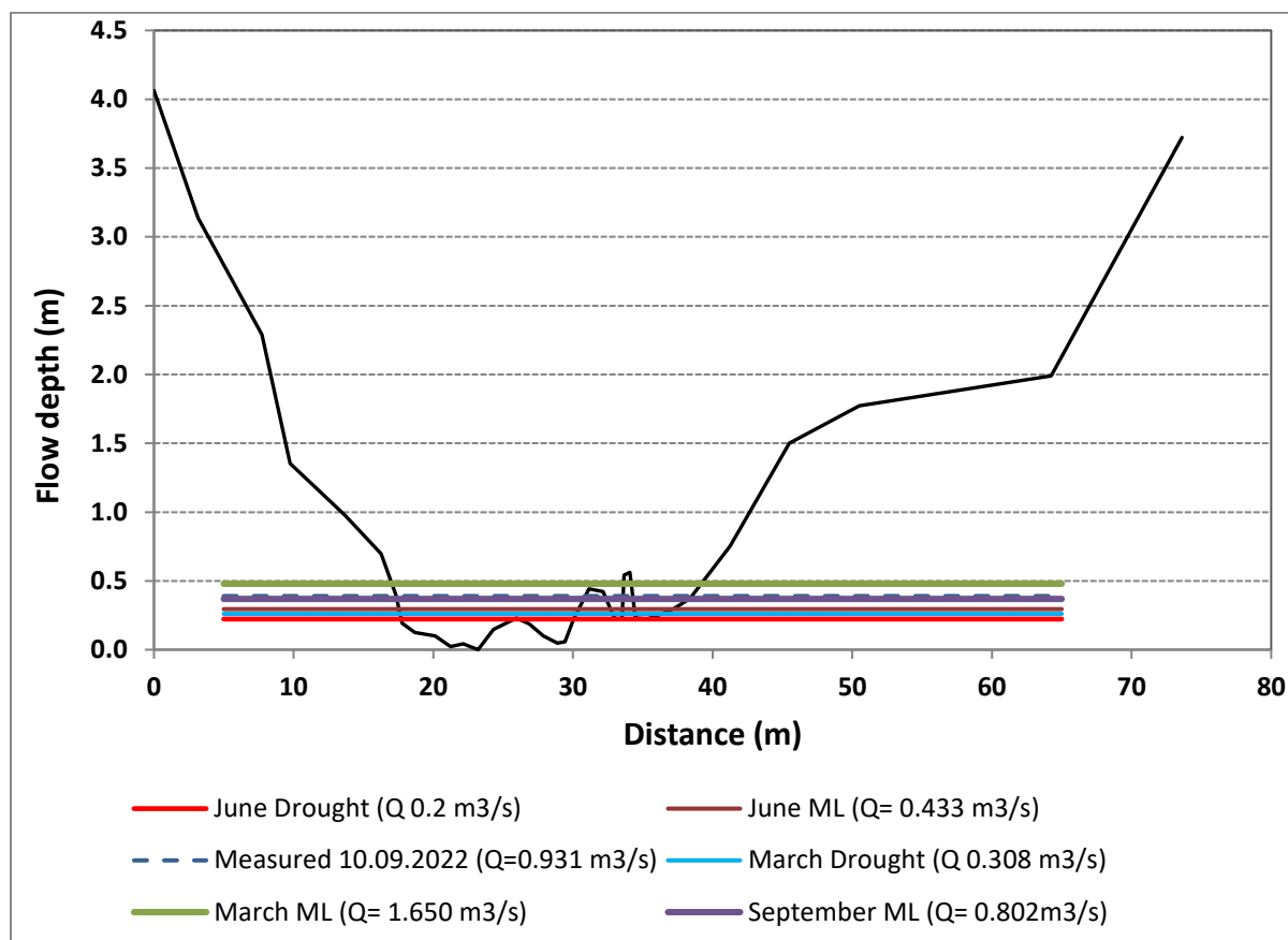
Figure 6-14: Water levels on cross-section of the EWR site for White Kei River in S10J.
