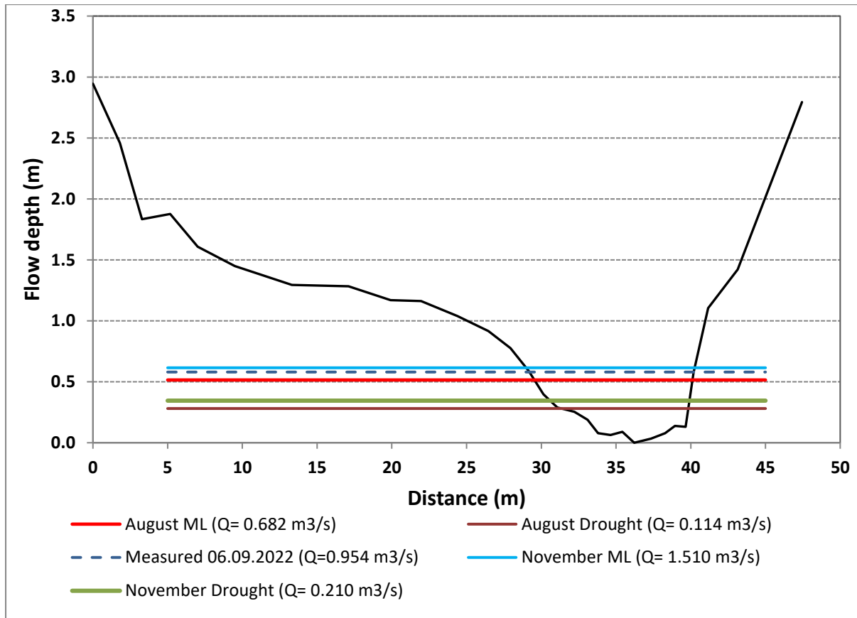
Figure 6-6: Water levels on cross-section of the EWR site for Mtentu River in T60C.
