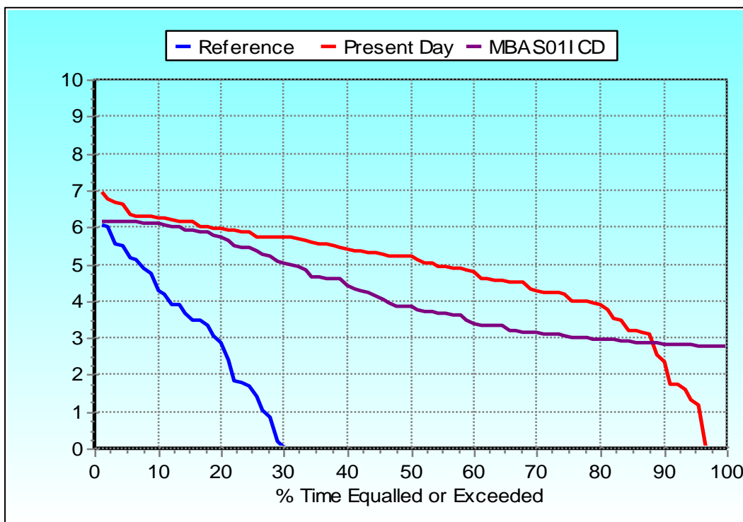
Figure 5-10: Final stress duration curves – wet season (March).
