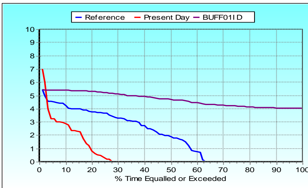
Figure 5-29: Final stress duration curves – dry season (June).
