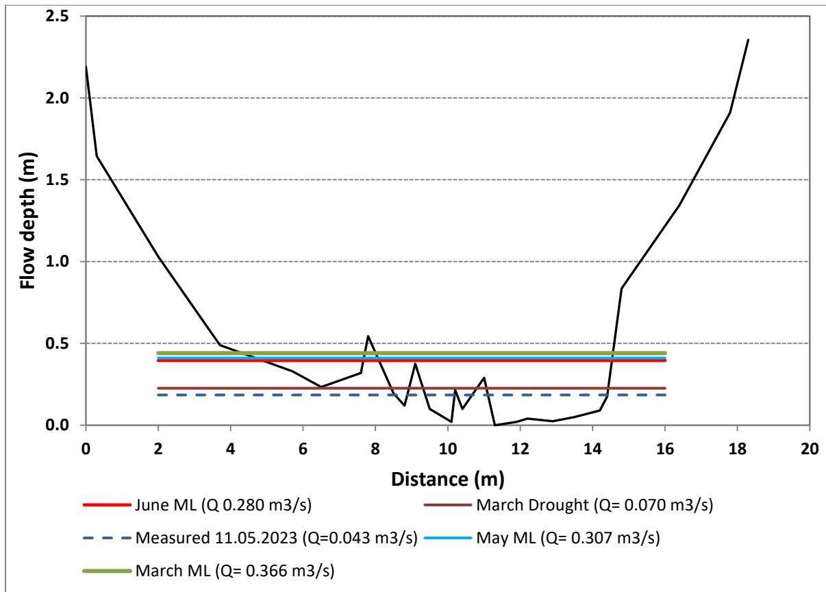
Figure 6-10: Water levels on cross-section of the EWR site for Gcuwa River in S70D.
