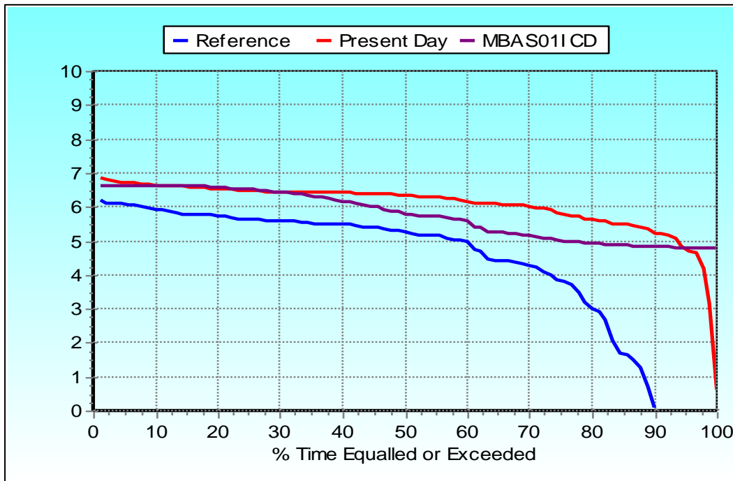
Figure 5-9: Final stress duration curves – dry season (June).
